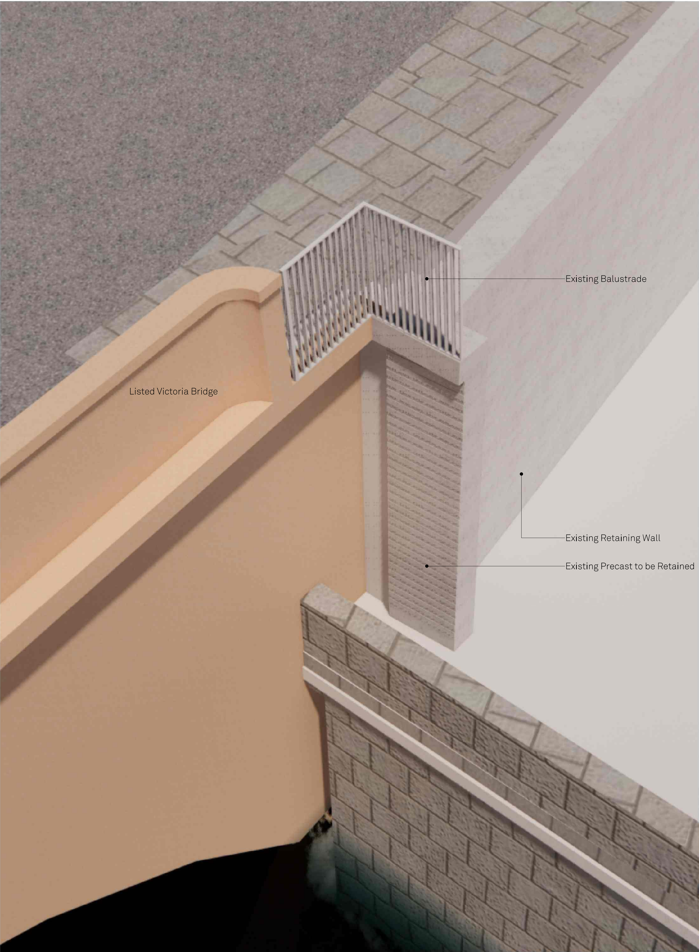
Existing Bridge Condition - Post Demolition
