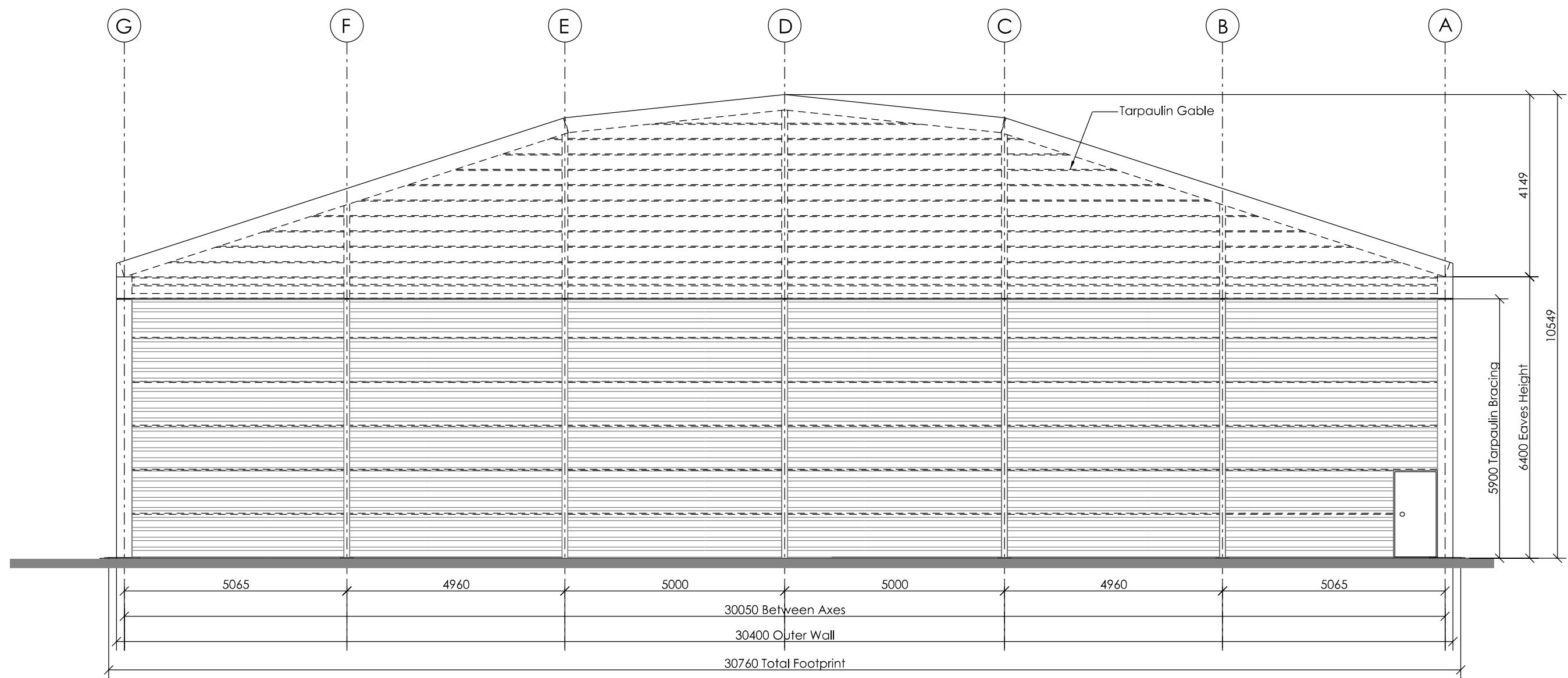
Rear (North) Elevation
