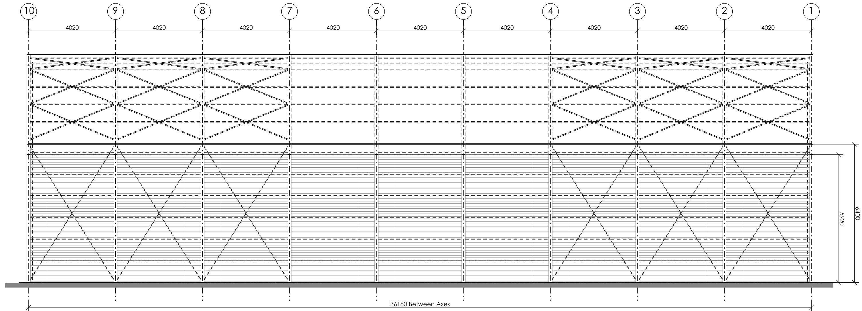
Side (West) Elevation
