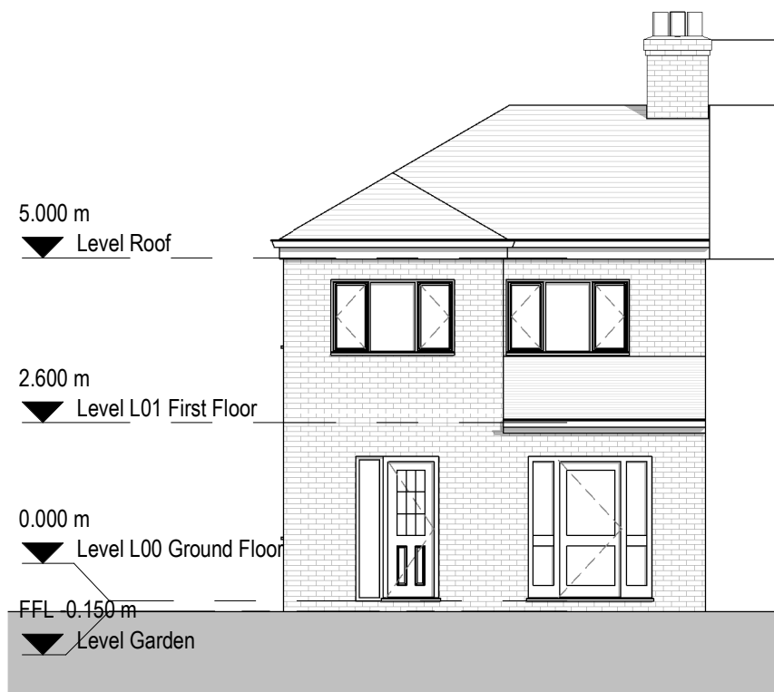
3 Existing North Elevation 1 : 100
