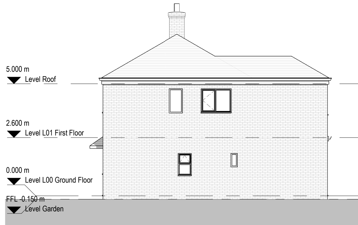
2 Existing East Elevation 1 : 100
