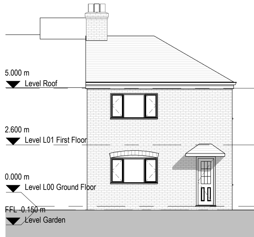
1 Existing South Elevation 1 : 100
