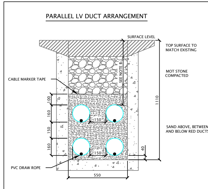
SECTION VIEW 'C' - DUCT ARRANGEMENT - SCALE 1:20
