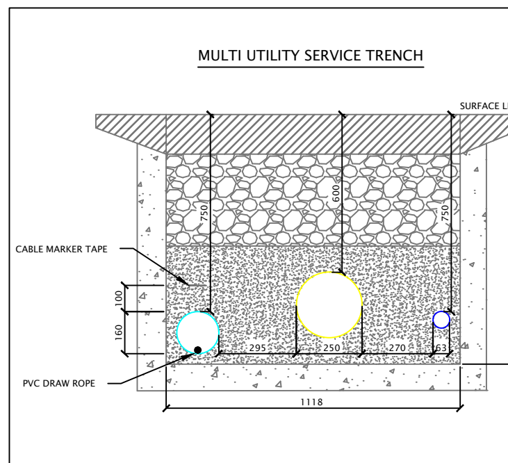
SECTION VIEW 'F' - SERVICE TRENCH ARRANGEMENT - SCALE 1:20
