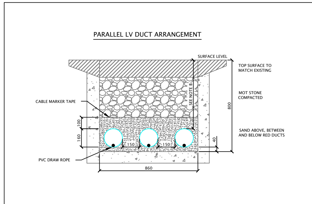
SECTION VIEW 'B' - DUCT ARRANGEMENT - SCALE 1:20
