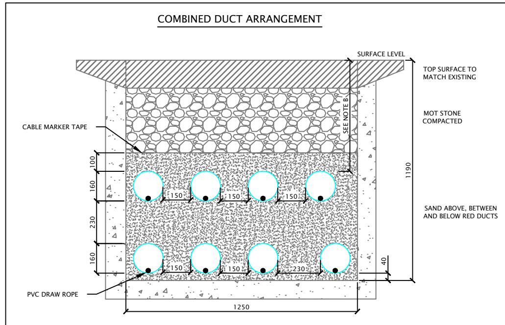
SECTION VIEW 'D' - DUCT ARRANGEMENT - SCALE 1:20
