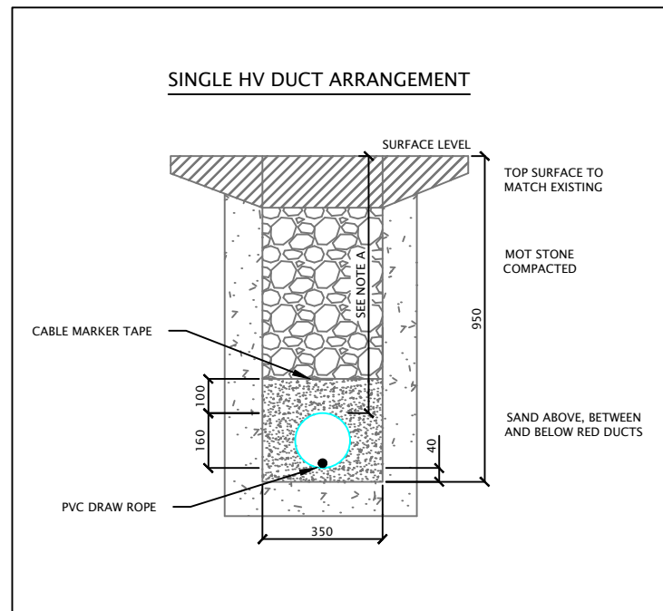
SECTION VIEW 'A' - DUCT ARRANGEMENT - SCALE 1:20
