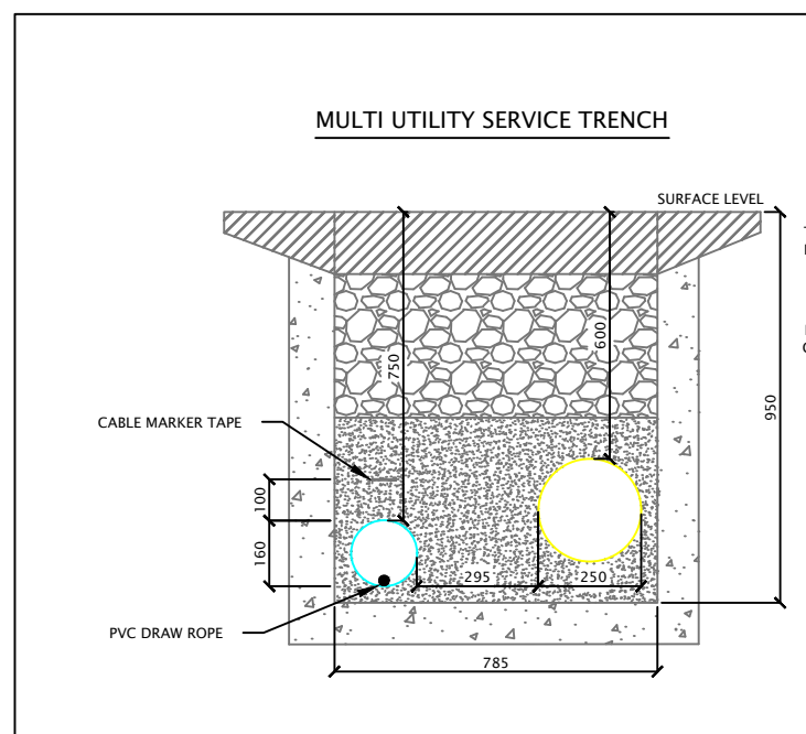
SECTION VIEW 'G' - SERVICE TRENCH ARRANGEMENT - SCALE 1:20
