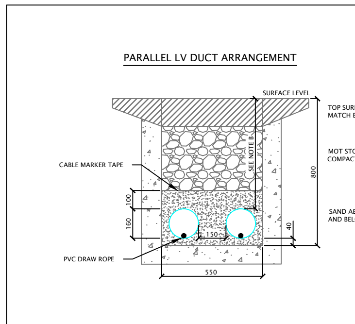
SECTION VIEW 'E' - DUCT ARRANGEMENT - SCALE 1:20
