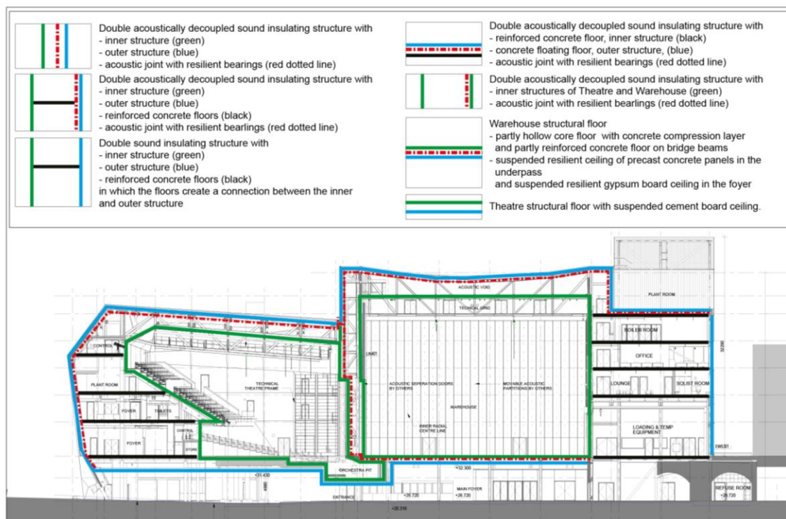
Figure 3: principle of sound insulating structures
