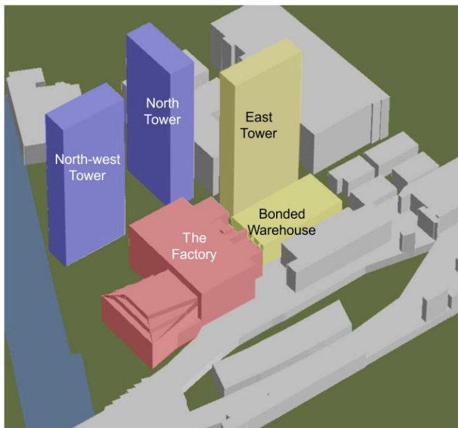
Figure 2: 3D noise model
