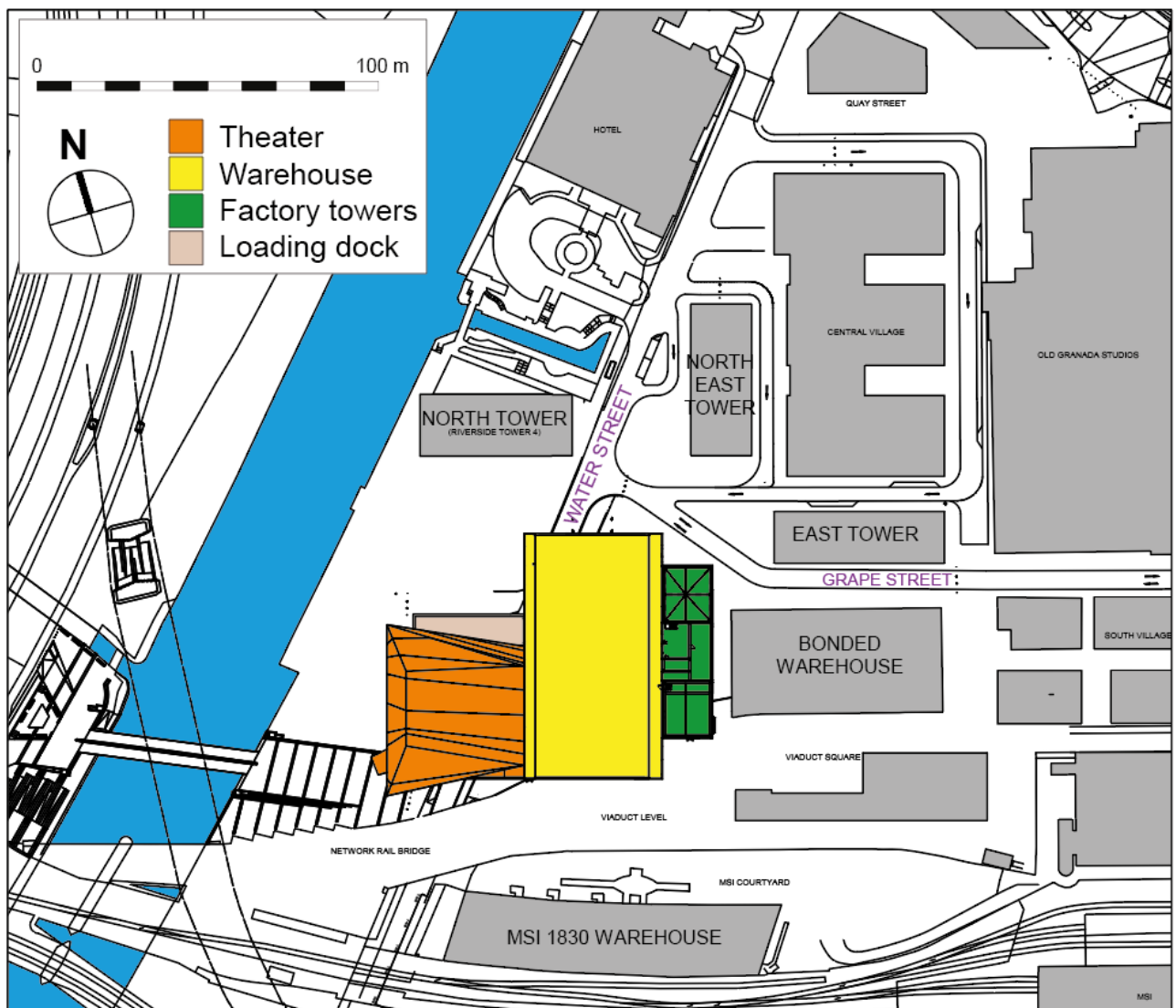
Figure 1: site plan in future context
