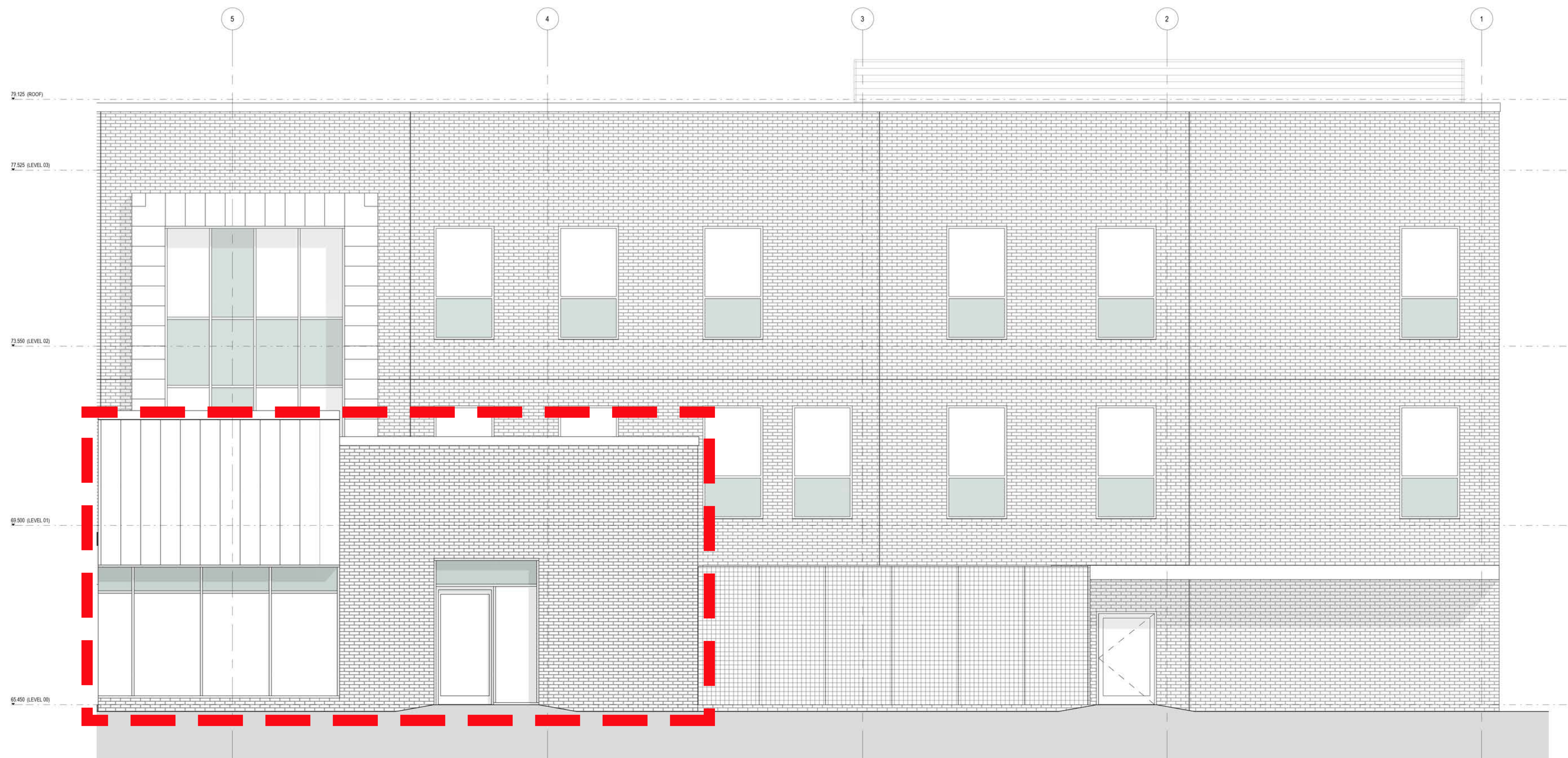
2 North Elevation 2 1:50
