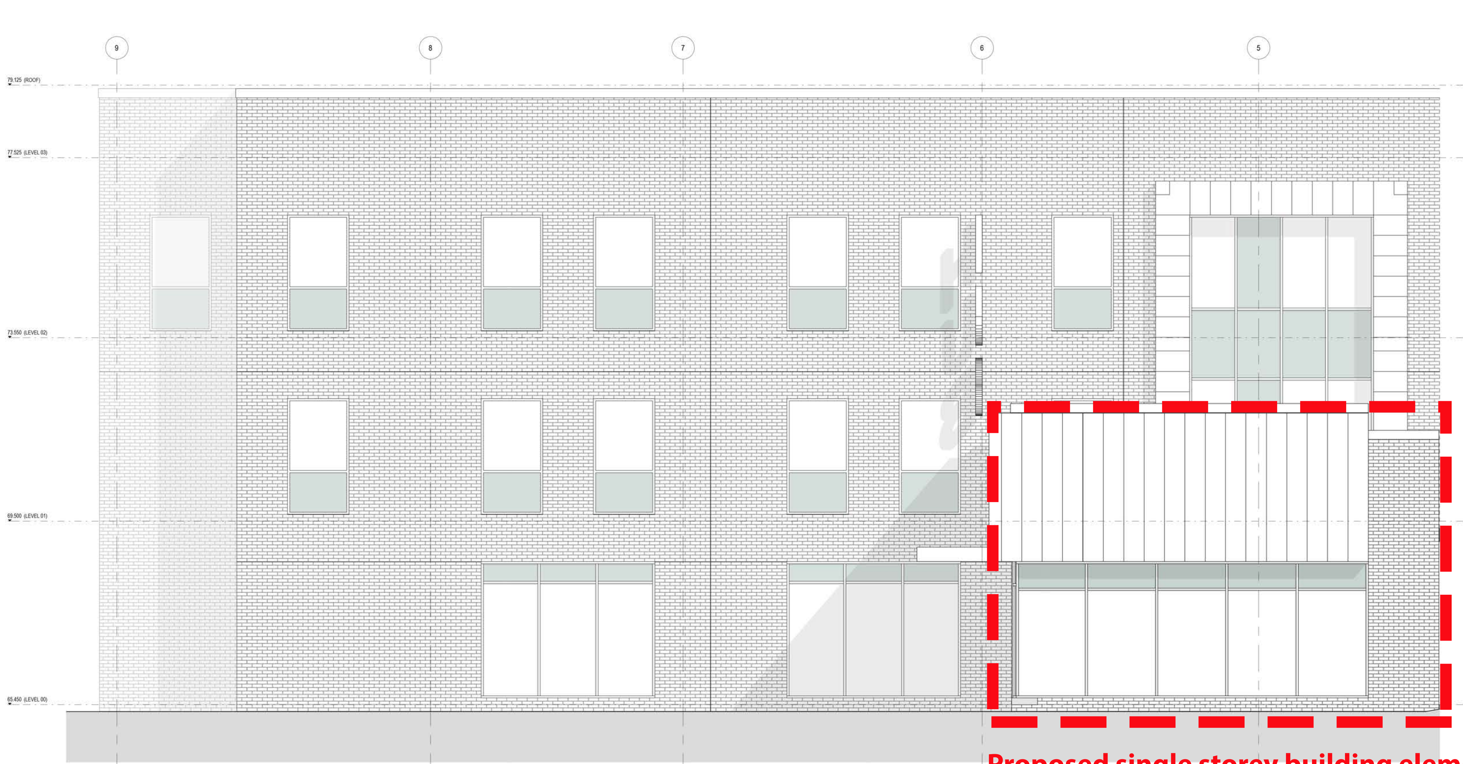
1 North Elevation 1 1:50
