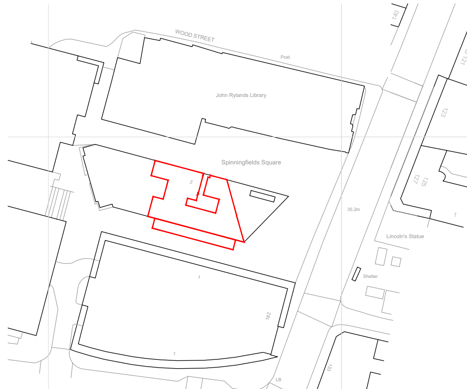
LOCATION PLAN
