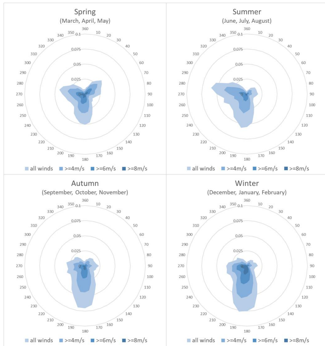
Figure 3: Seasonal Wind Roses for Manchester International Airport
