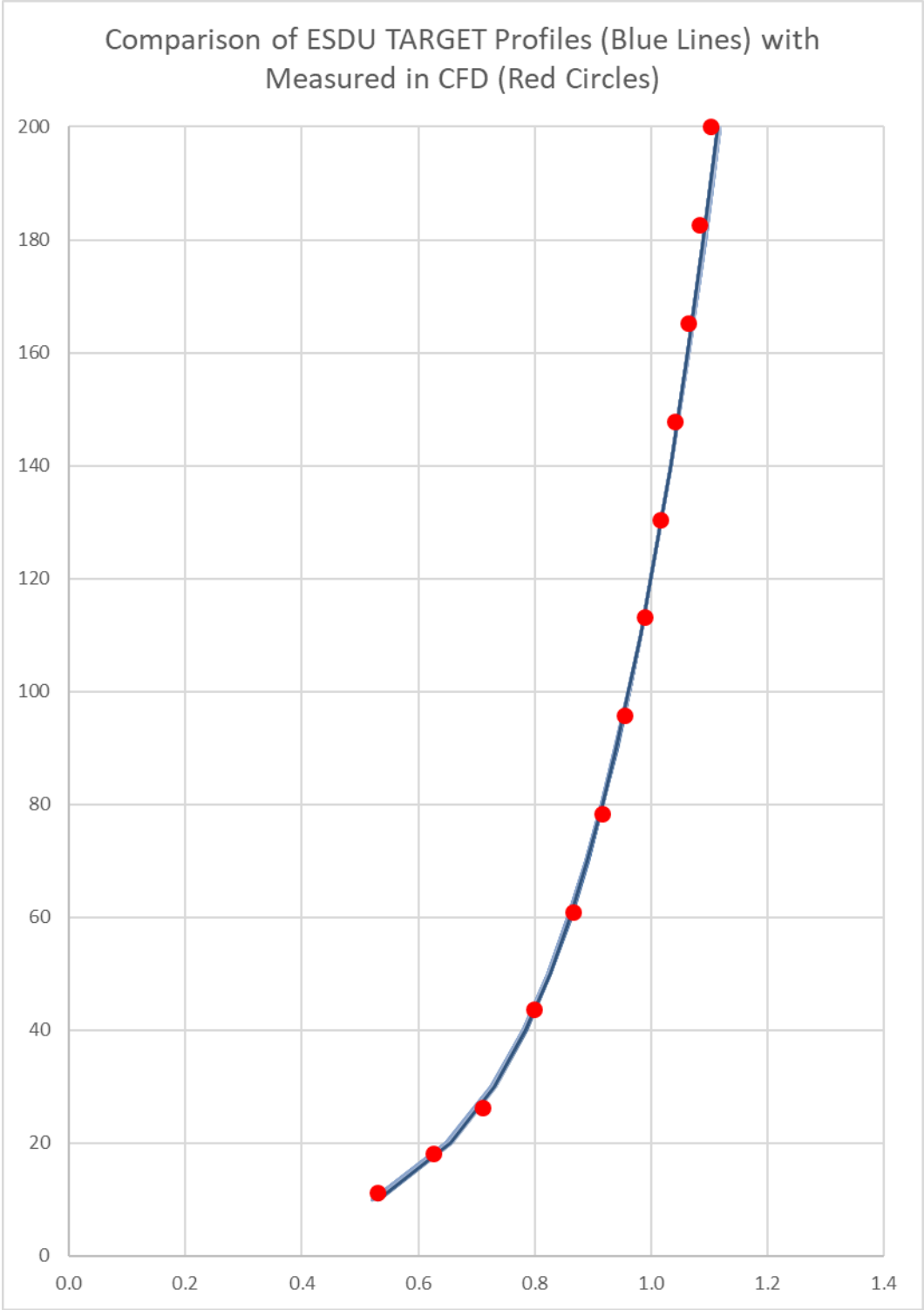
Figure 4: Wind Profile for Boddingtons
