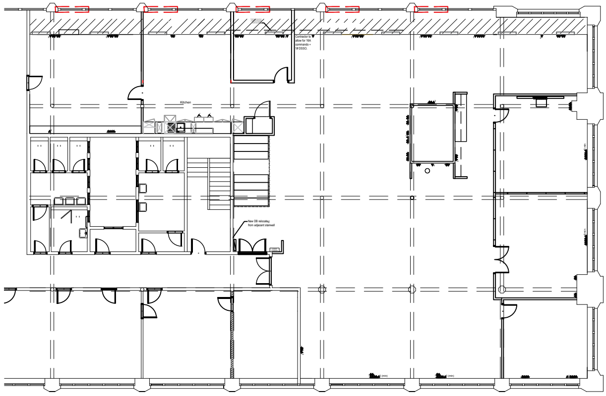
ACTUATOR LOCATION PLAN Scale 1:200
