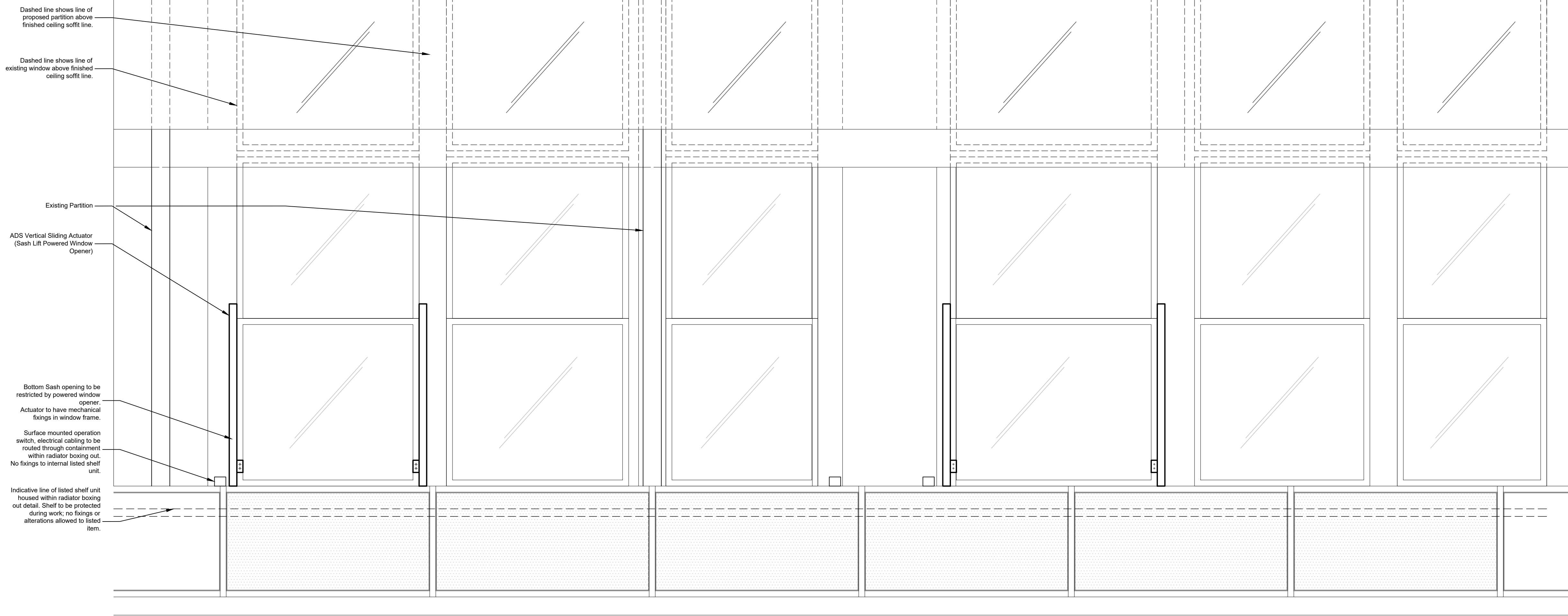
ELEVATION Scale 1:16
