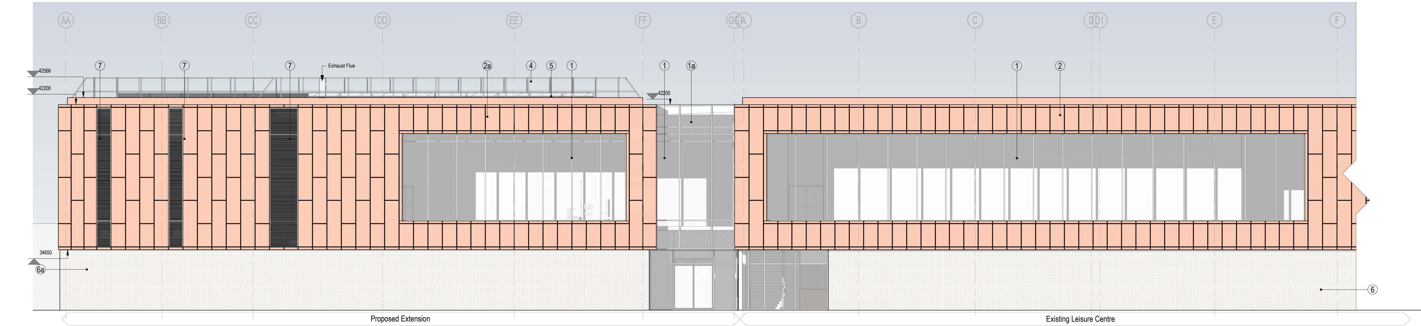
2 | Elevation 02 - East
