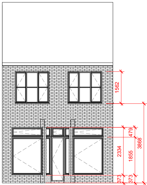
1 Front Existing 1 : 100
