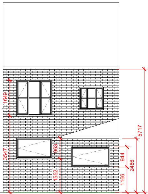
3 Rear Existing 1 : 100
