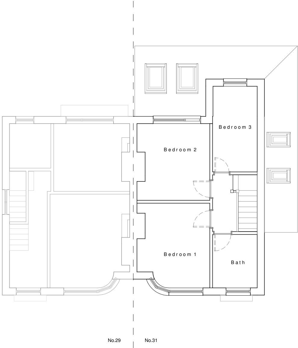
Level 1 as Proposed
