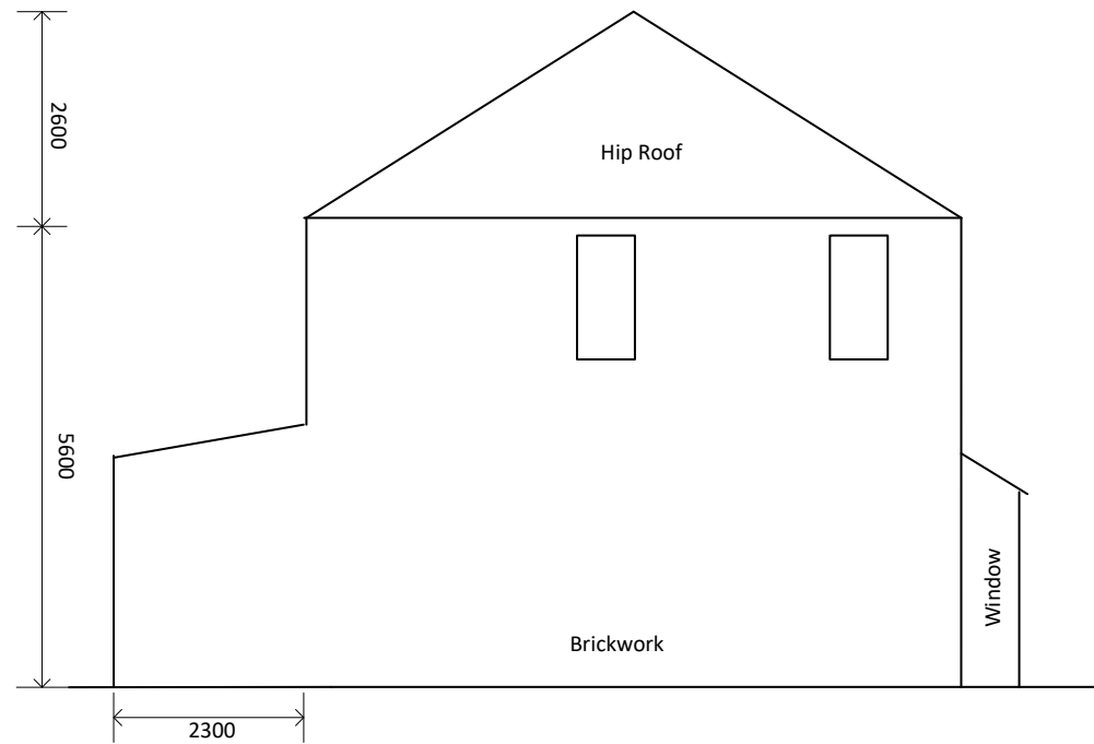
EXISTING SIDE ELEVATION (from H. No. 76)
