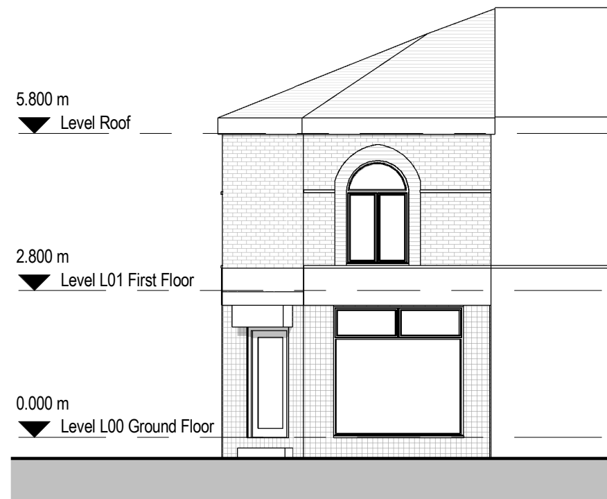
1 Existing West Elevation 1 : 100
