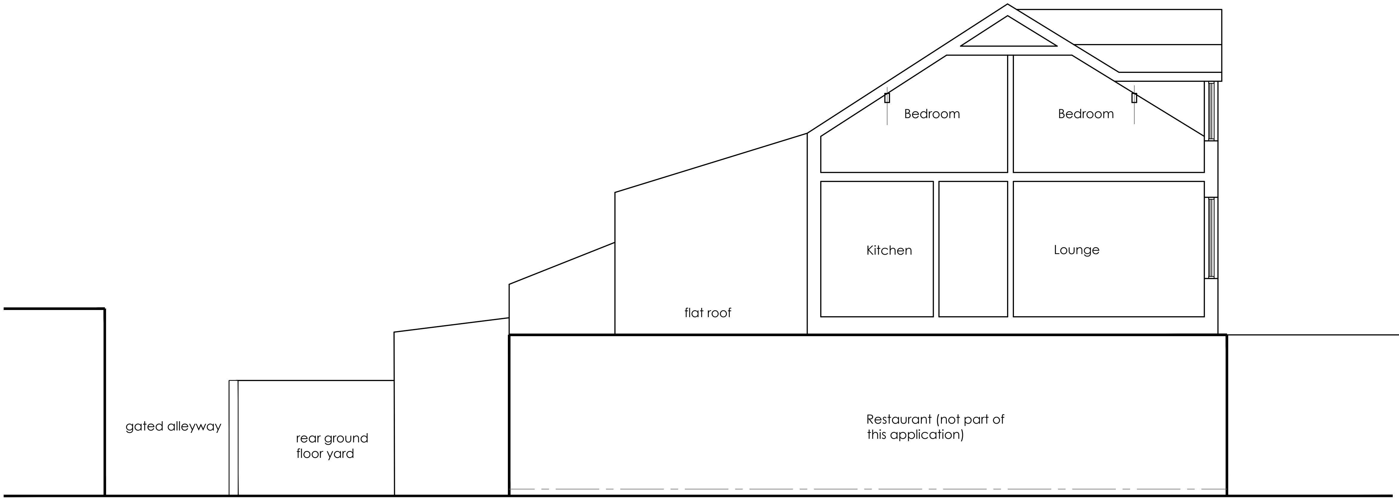
EXISTING CROSS SECTION
