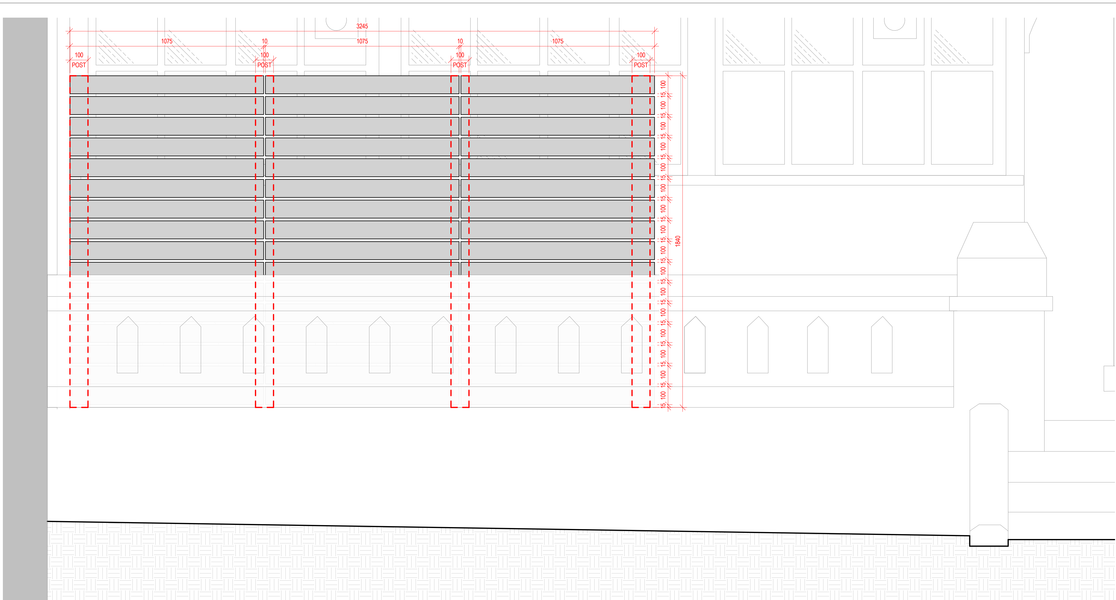
South Facing Elevation 1 : 10
