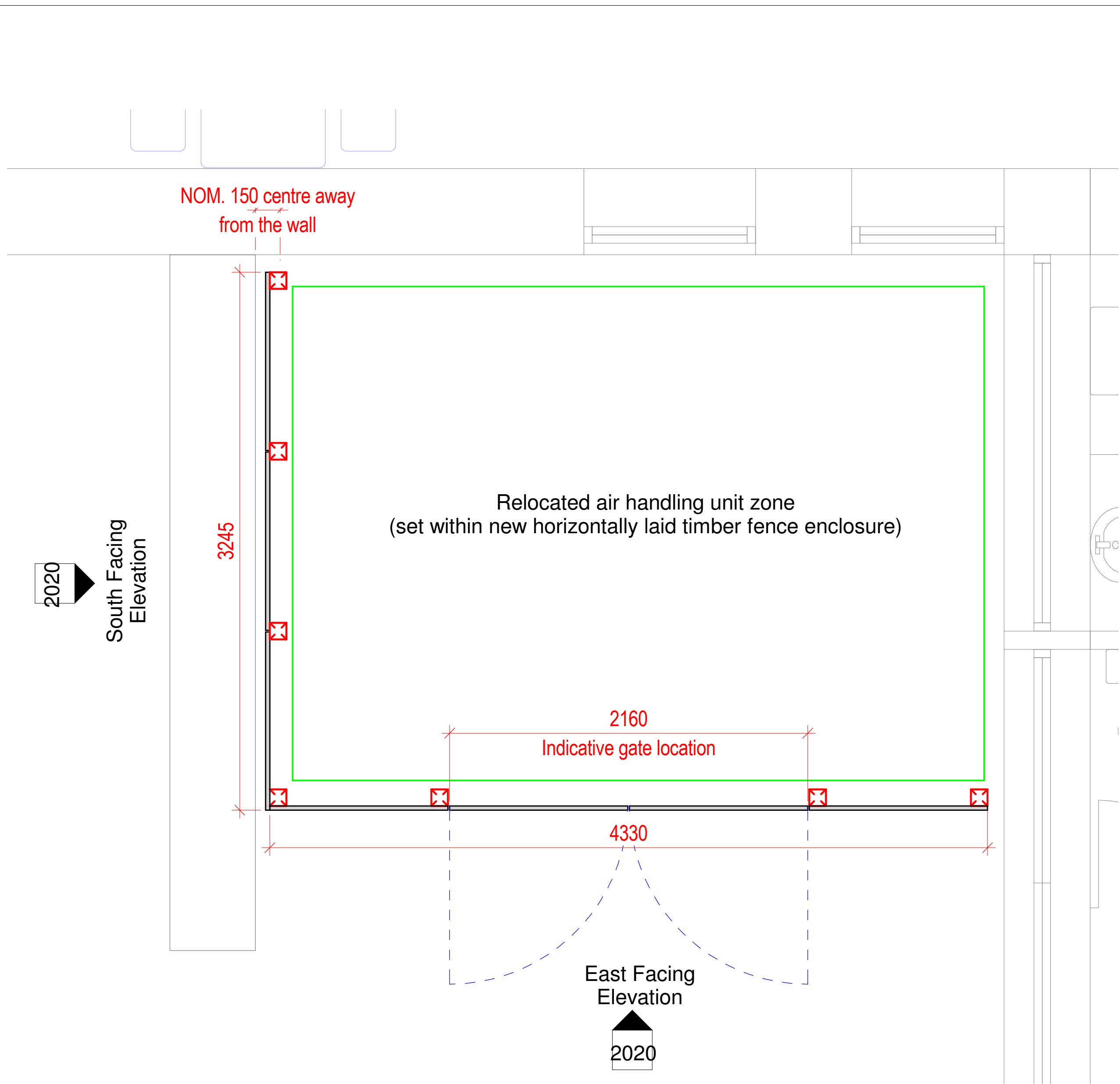
Plant Enclosure - Plan Detail 1 : 20
