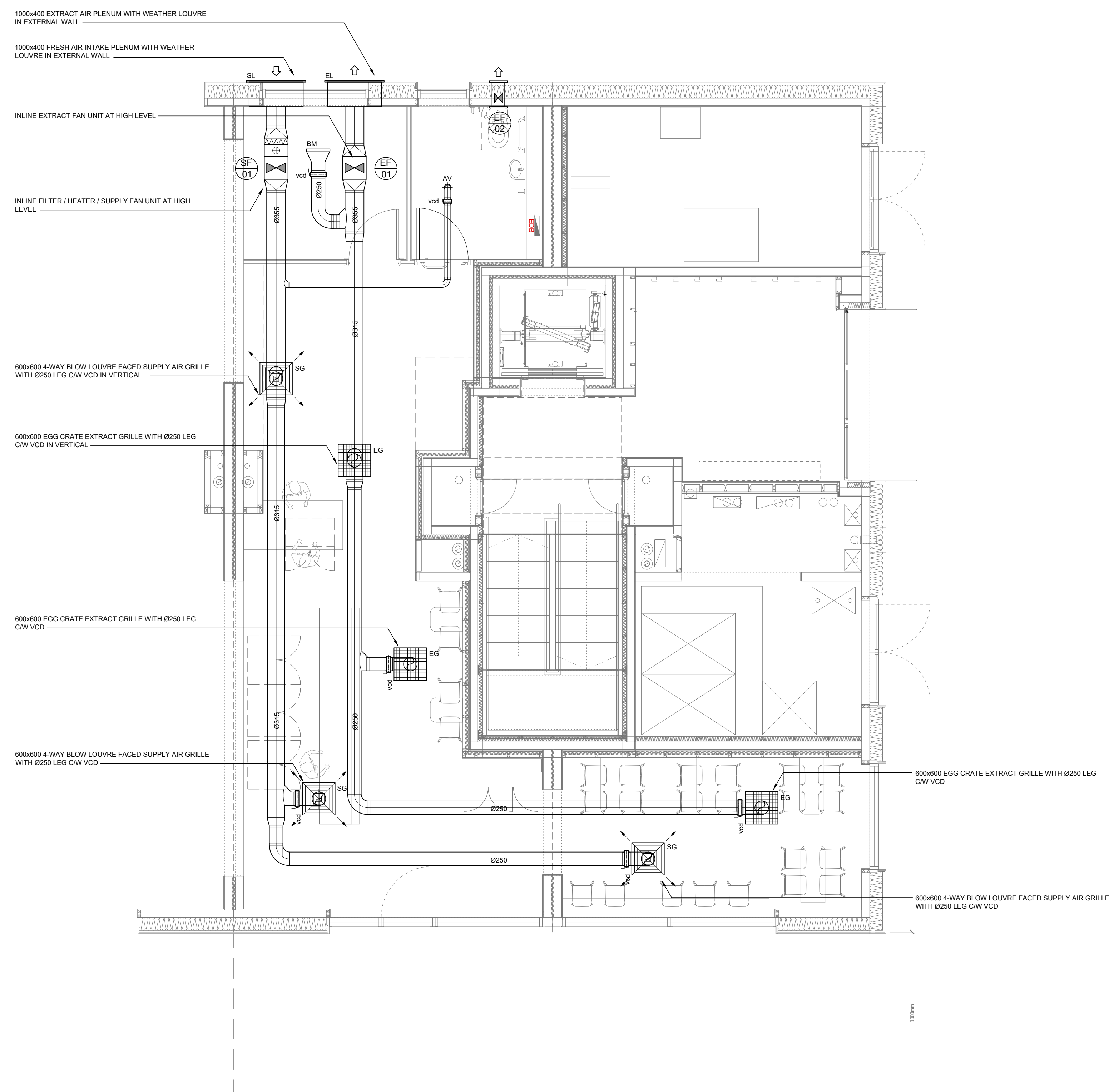
PLAN AT GROUND FLOOR LEVEL Scale 1:50
