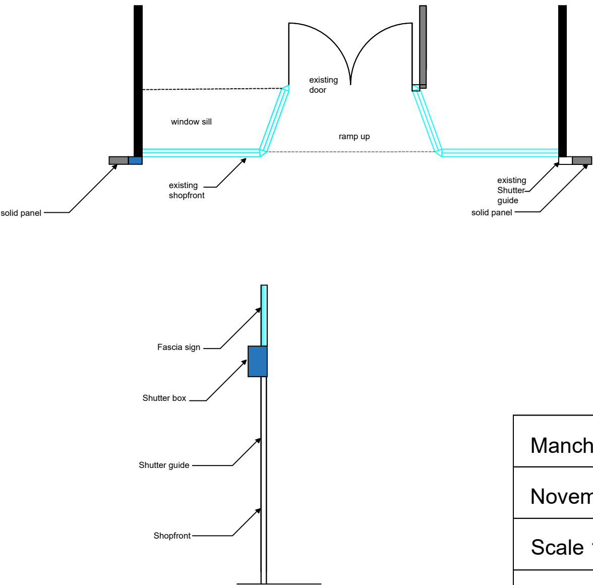
Proposed Shopfront - side elevation
