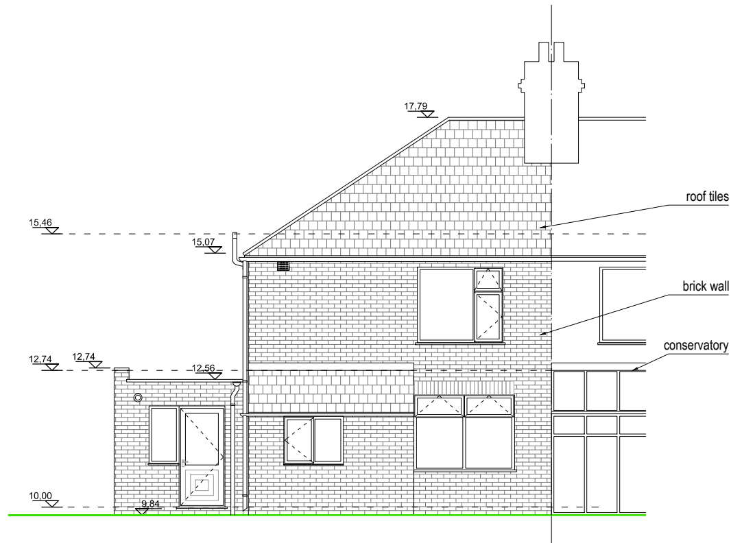
SOUTH ELEVATION
