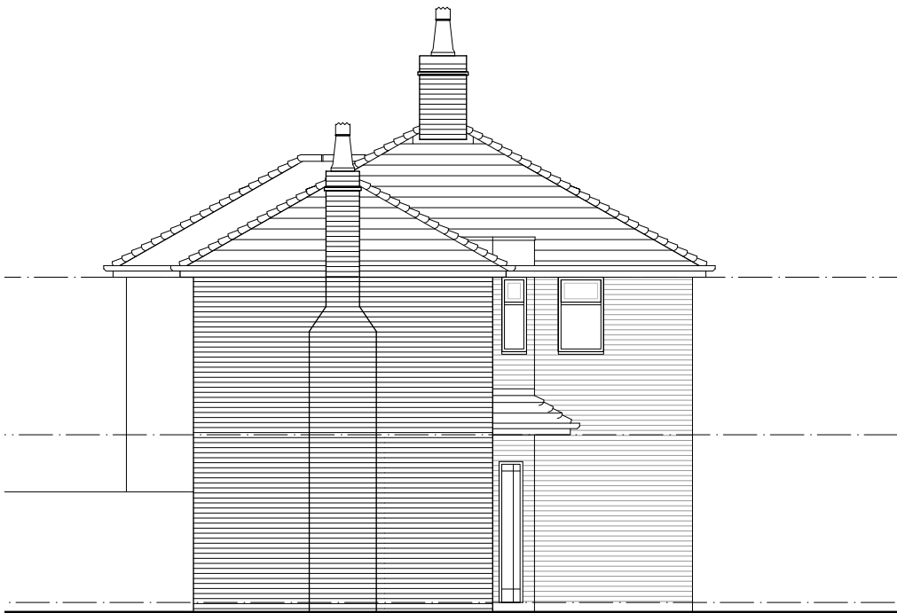
Side Elevation (No.30)
