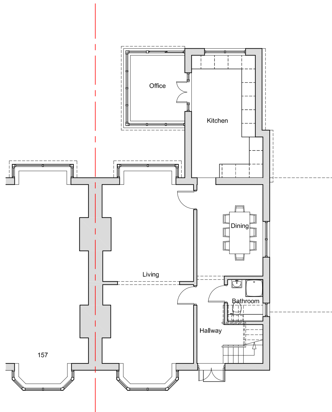
Proposed G/F Plan 1:100
