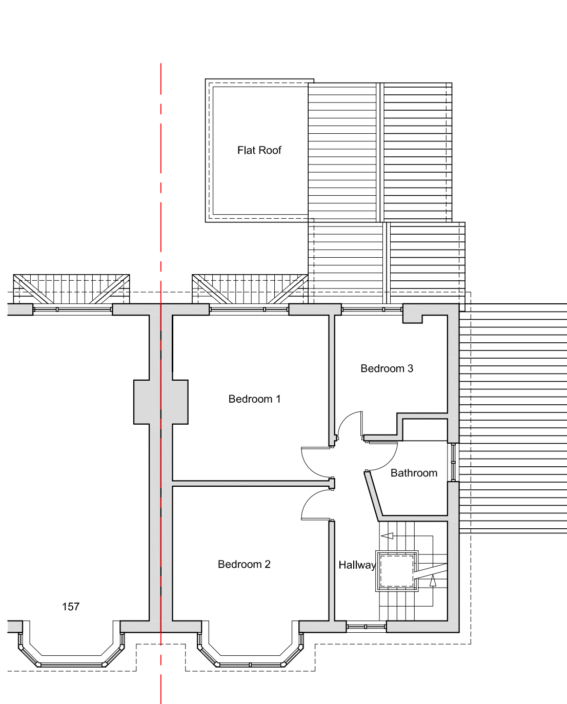
Proposed 1/F Plan 1:100
