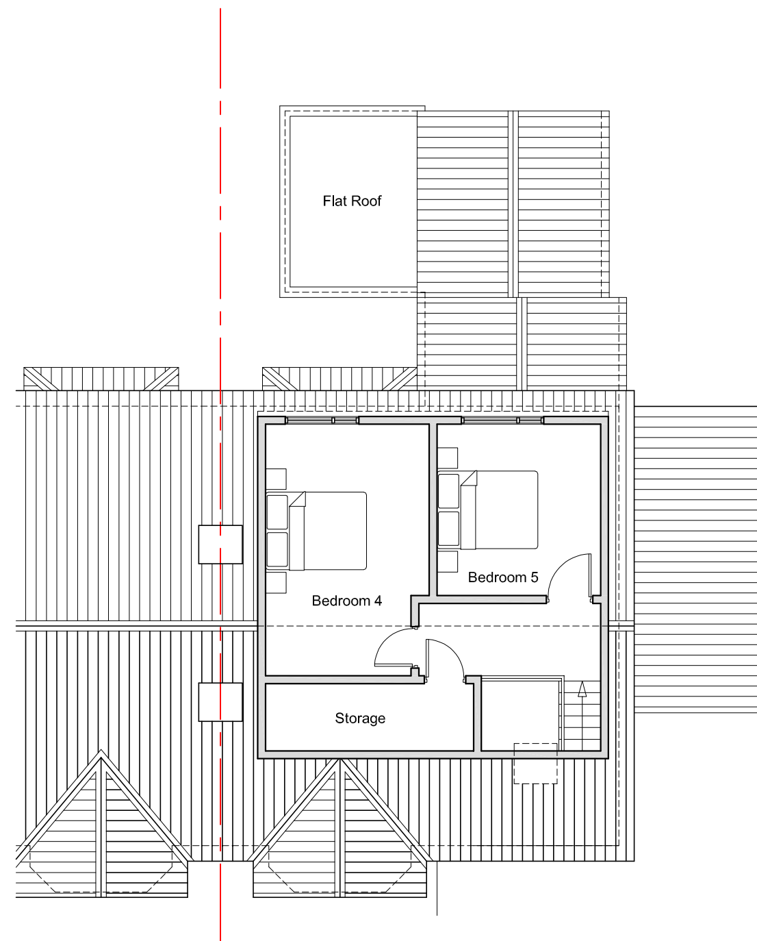
Proposed Loft Plan 1:100
