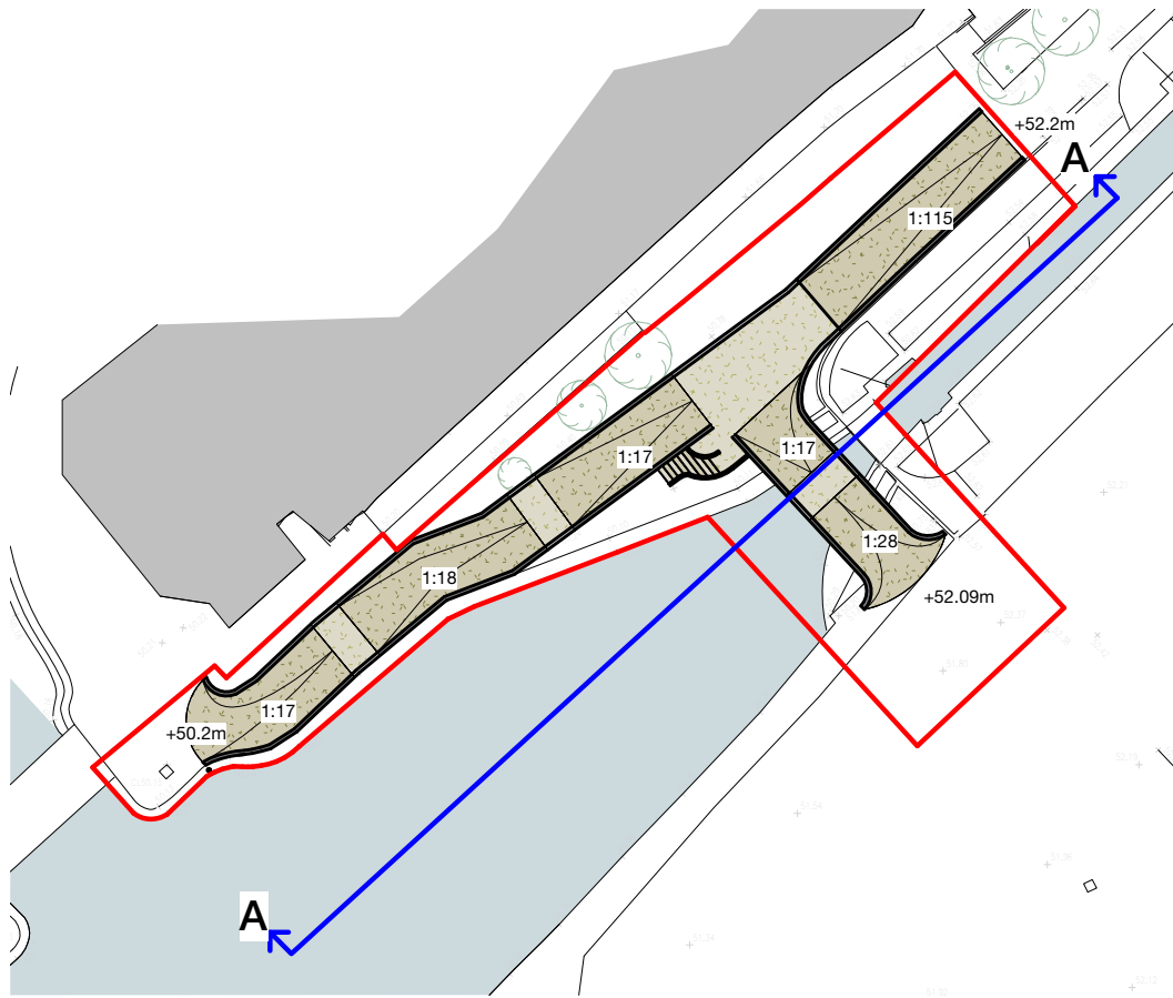
Proposed Elevation A-A Reference Plan 1 : 500
