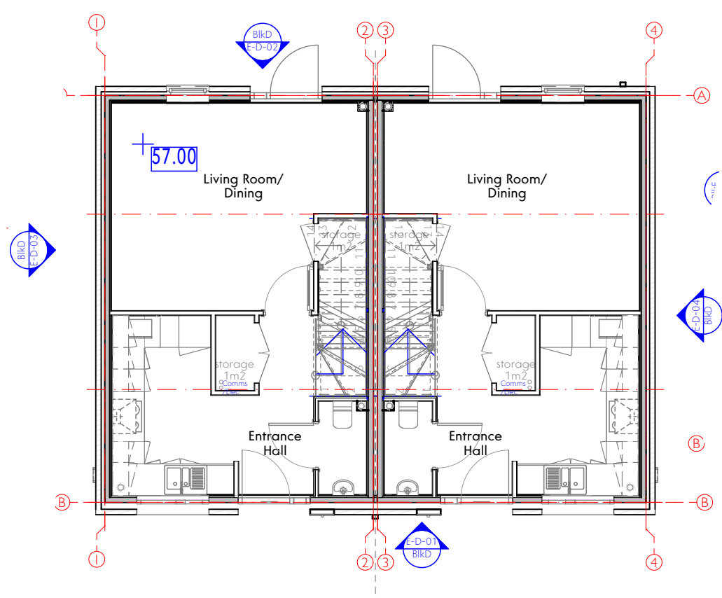
Block D-Ground Floor 2x 2b3p Dwellings
