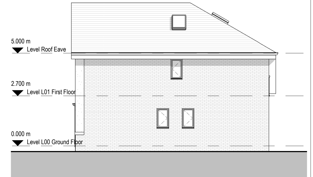
4 Proposed North Elevation 1 : 100
