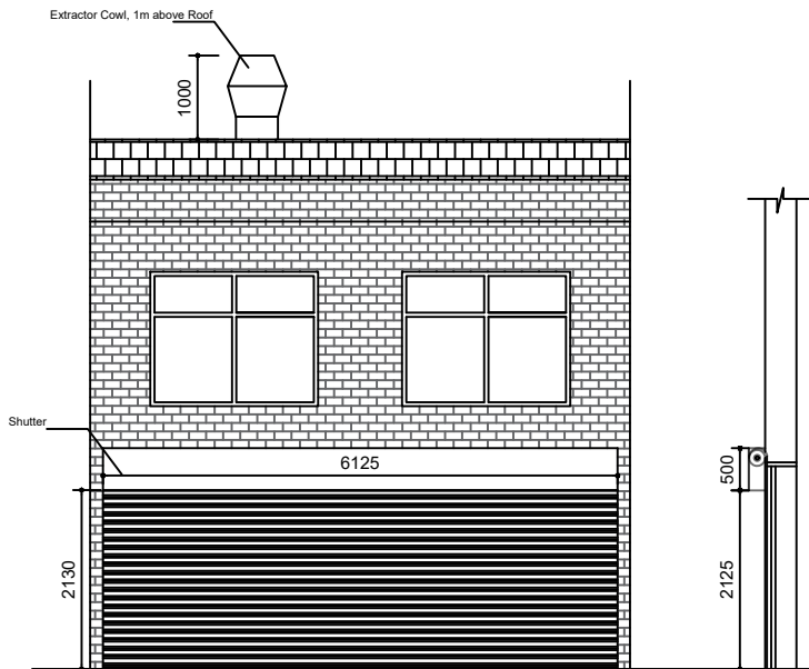
PROPOSED SHUTTER
