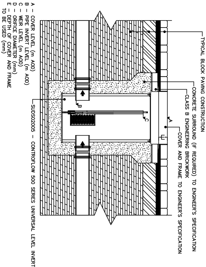
SUDS02005 – CONTROLFLOW 500 SERIES UNIVERSAL LEVEL INVERT GENERAL APPLICATION
