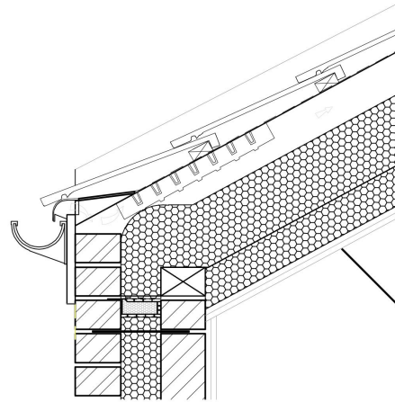
EAVES DETAIL
