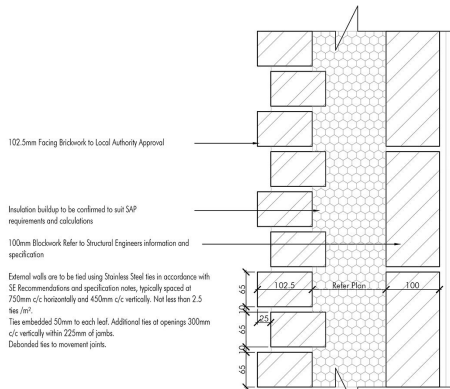
BRICK FEATURE DETAIL
