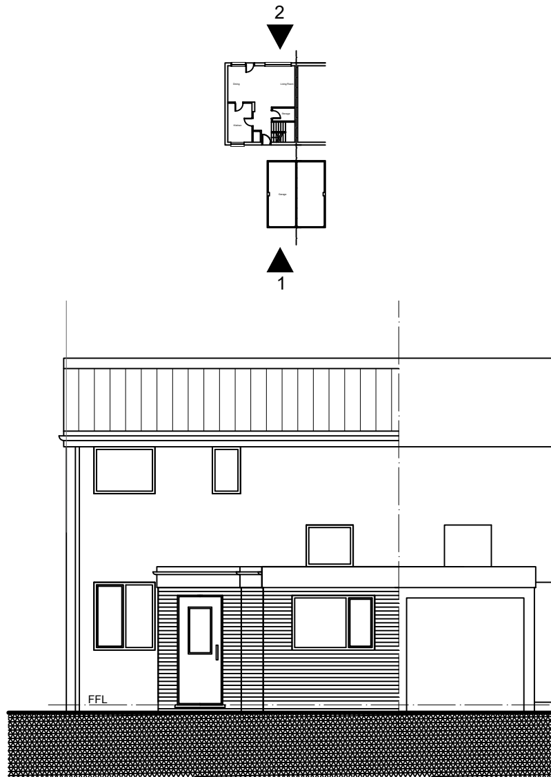
Proposed Elevation 1
