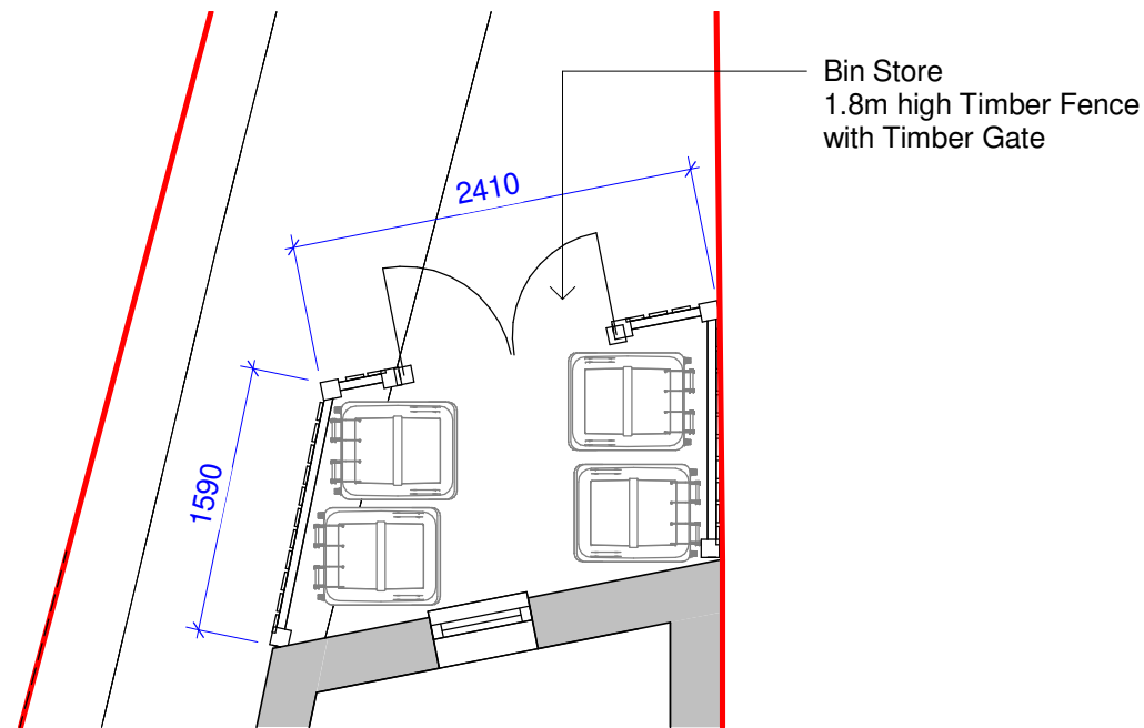
1 Proposed Bin Store Plan 1 : 50
