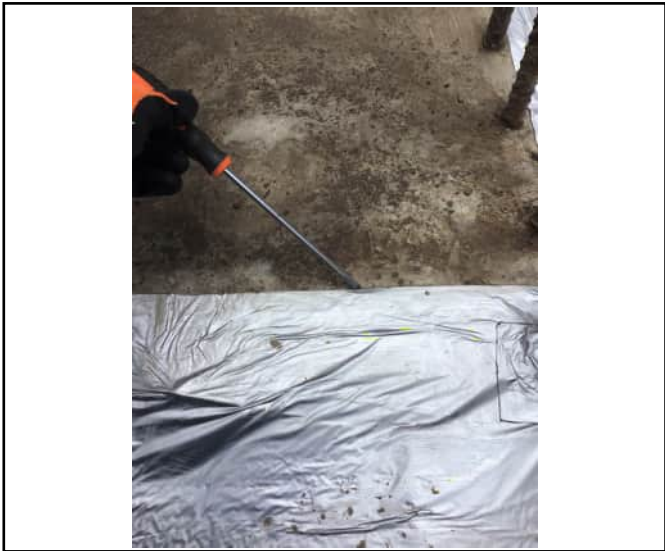
Pick and probe test carried out
