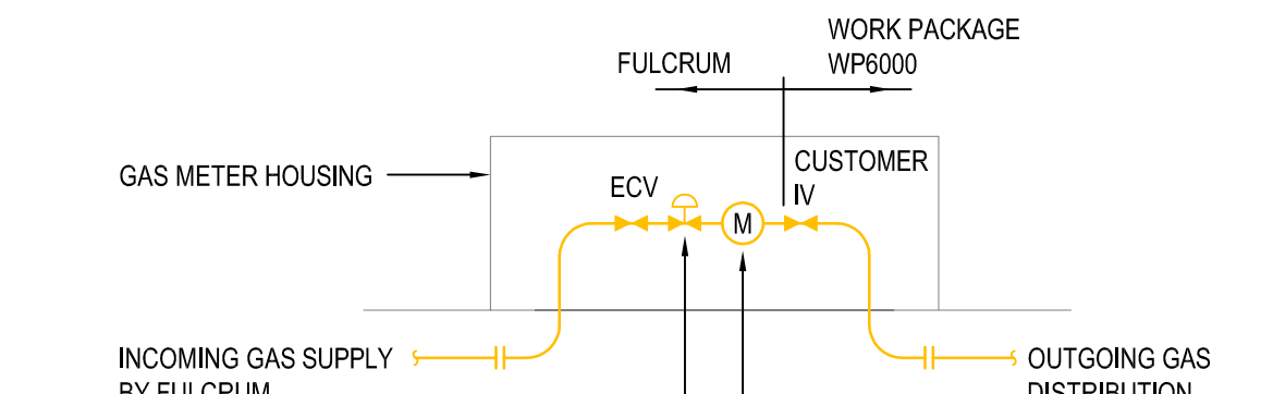
PROPOSED ARRANGEMENT OF GAS SUPPLY ARRANGEMENTS AT FULCRUM
