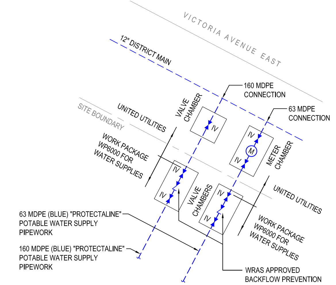
PROPOSED ARRANGEMENT OF POTABLE WATER AND FIRE FIGHTING WATER SUPPLY CONNECTIONS AT SITE BOUNDARY
