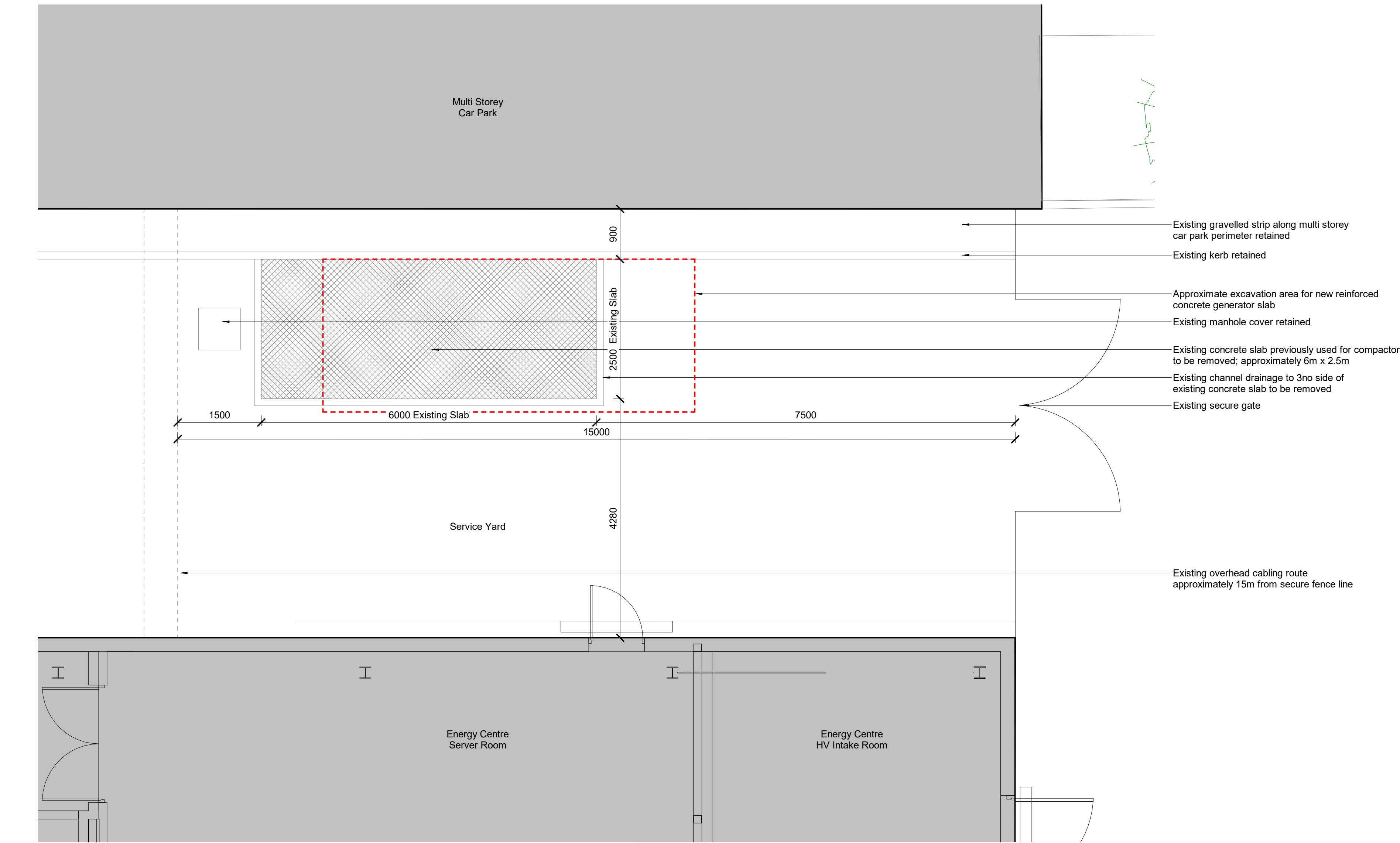
1 Energy Centre - Existing GA Plan 02101 1 : 50
