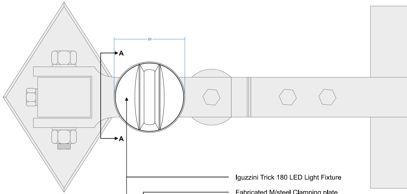
Hinge Mount Front View Scale 1:1 @ A0
