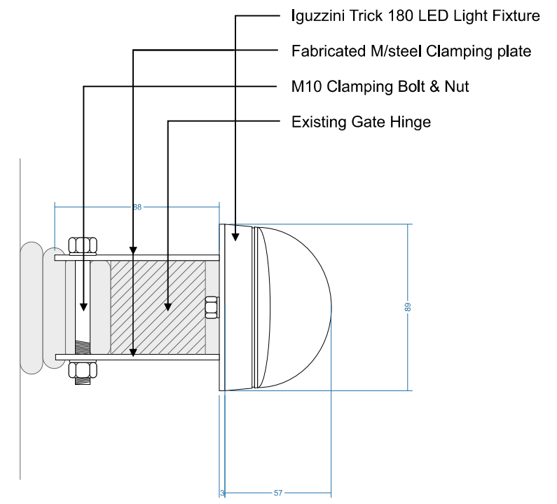
Hinge Mount Section A-A Scale 1:1 @ A0
