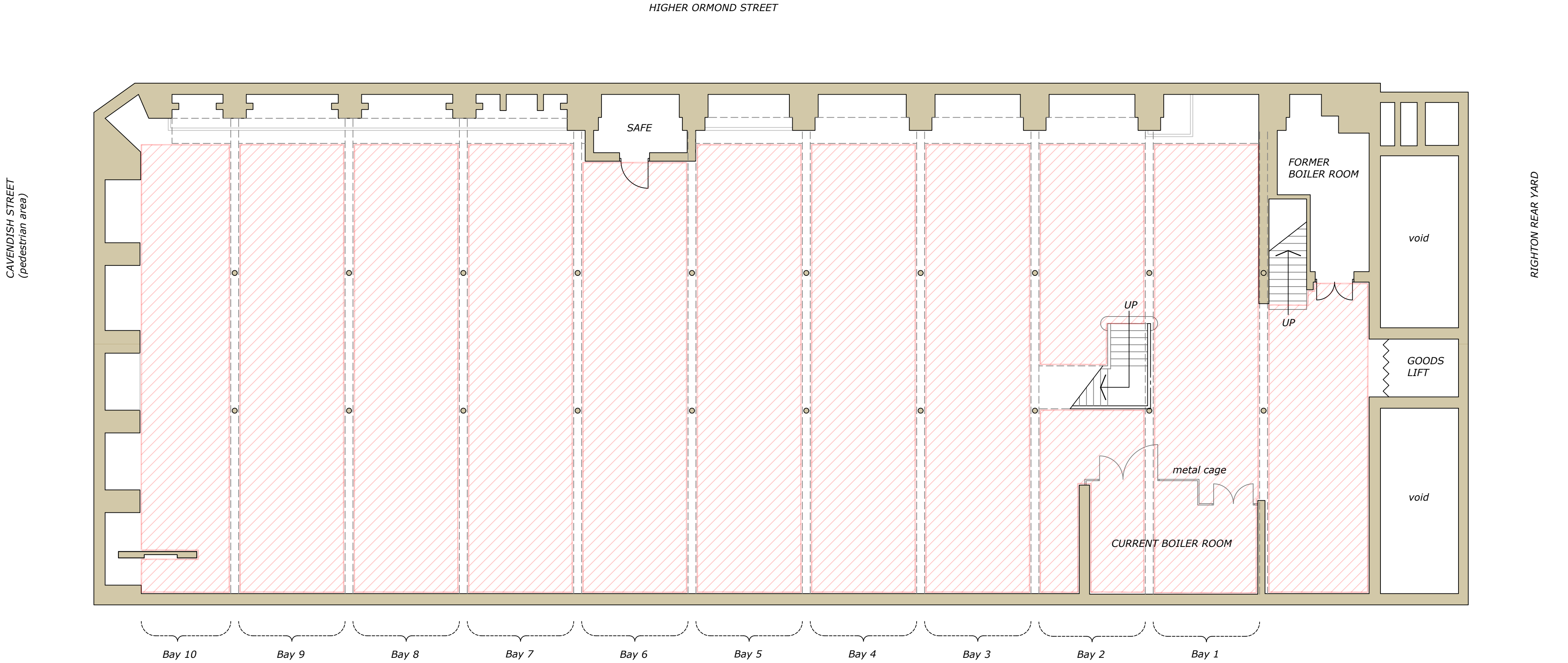
Righton Basement Plan (scale 1:100)
