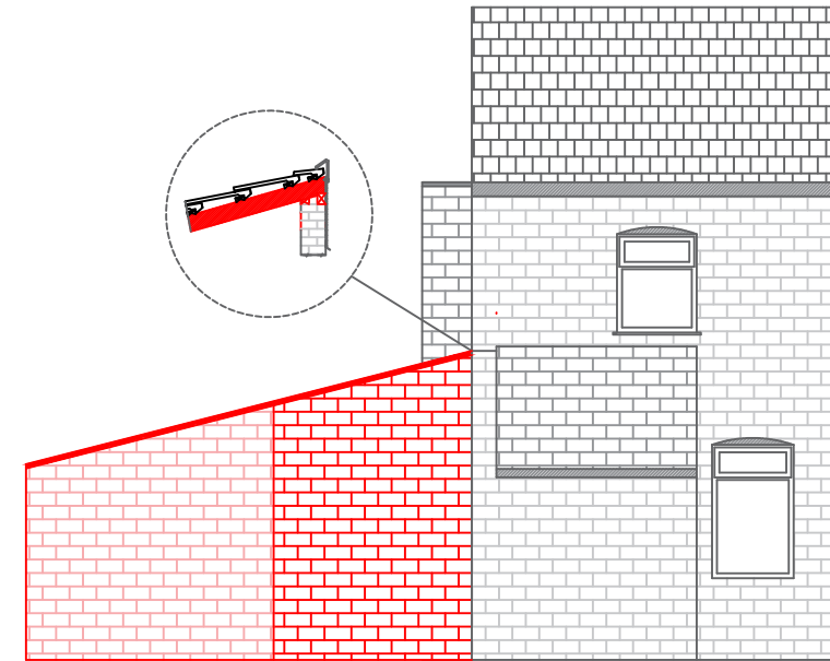
Proposed Rear Layout
