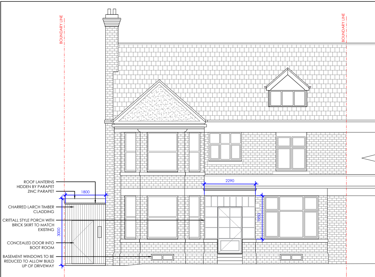
E PROPOSED FRONT ELEVATION 1:100
