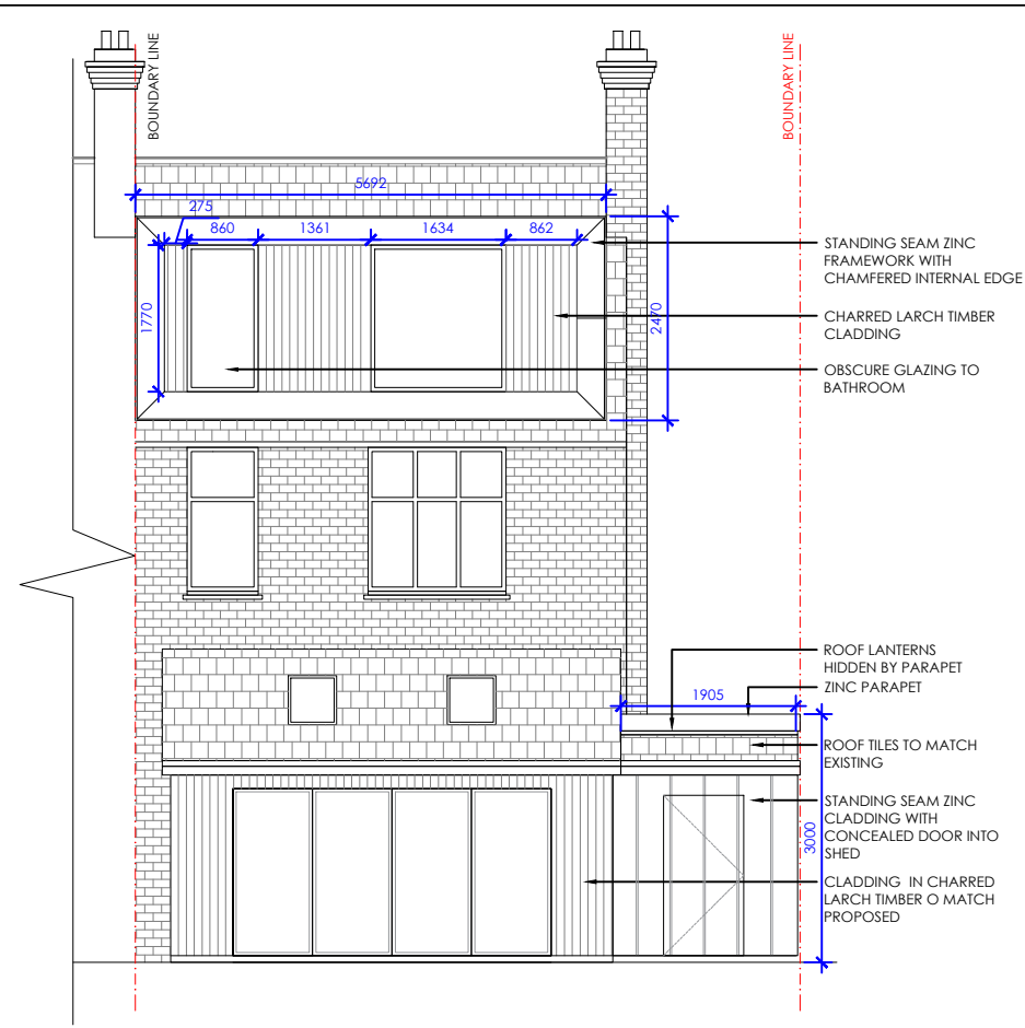
E PROPOSED REAR ELEVATION 1:100
