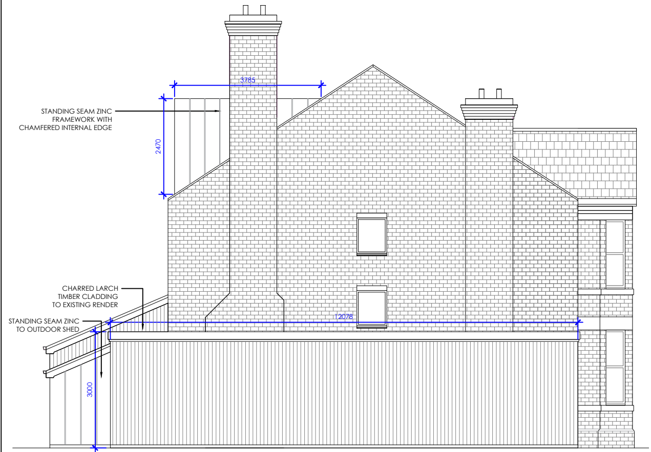
E PROPOSED FRONT ELEVATION 1:100
