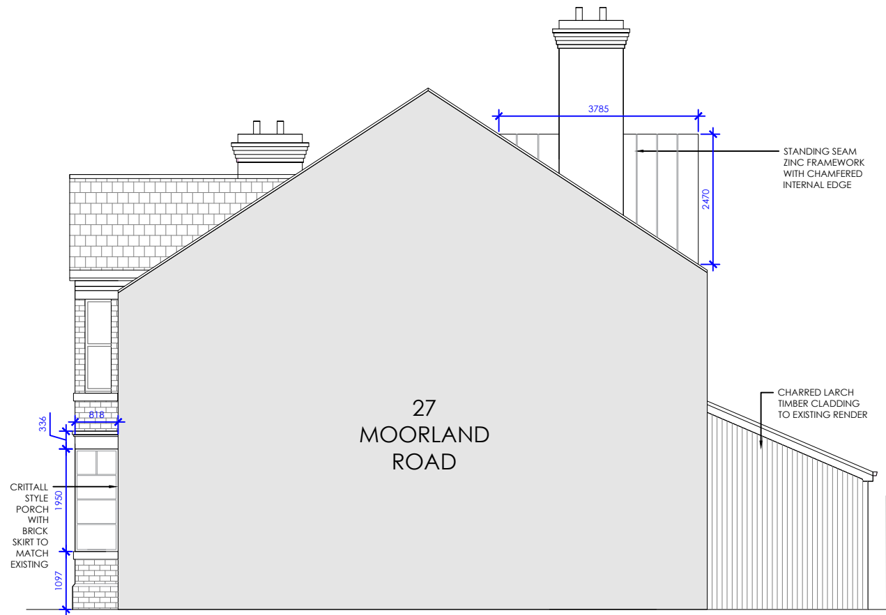
E PROPOSED SIDE ELEVATION 1:100
