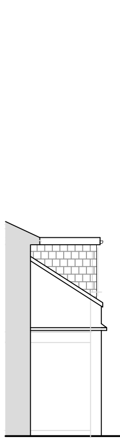
Proposed RH Side Elevation (Viewed from Rear Elevation)
