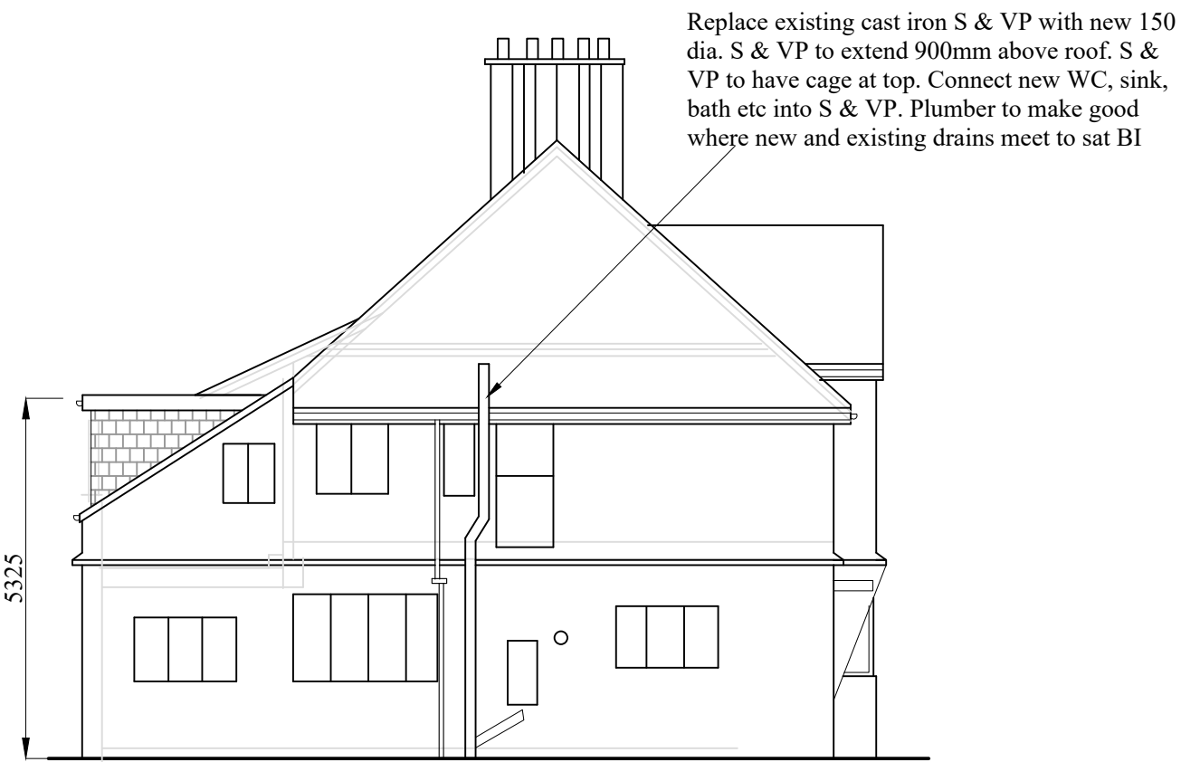
Proposed LH Side Elevation
