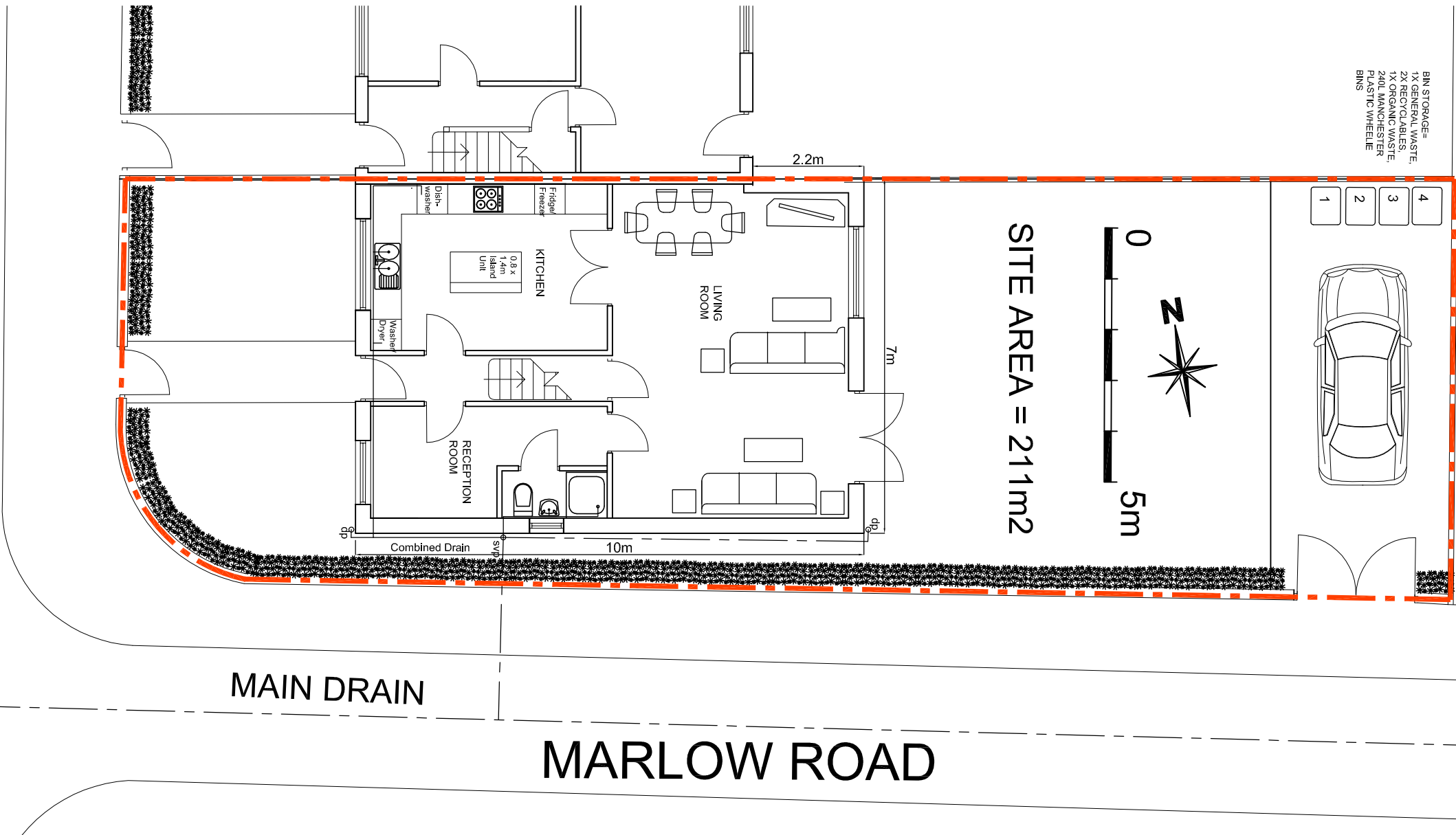
The floor plan illustrates a residential unit with the following layout and features: Overall Dimensions: The unit measures 10m in width and 7m in depth. Kitchen: Located at the top left, it includes a Fridge/Freezer, Dishwasher, and a 0.8 x 1.8 Island Unit. The area is labeled 4650. Living Room: Situated at the top right, it features a sofa, armchairs, and a coffee table. The area is labeled 4650. Reception Room: Located at the bottom right, it contains a sofa, armchairs, and a coffee table. Hall: Centrally located, it provides access to the other rooms and includes a staircase. Bathroom: Located at the bottom left, it contains a toilet, sink, and bathtub. Washing Area: Adjacent to the kitchen, it includes a Washer and Dryer. Drainage: A Combined Drain is shown at the bottom left, and an SVP (Sewer Vent Pipe) is indicated near the bathroom.
