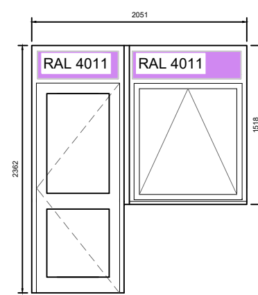
12 X Type K Window
