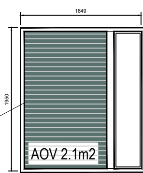
12 X Type C Window
