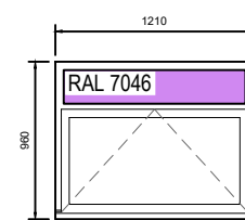
2 X Type F Window
