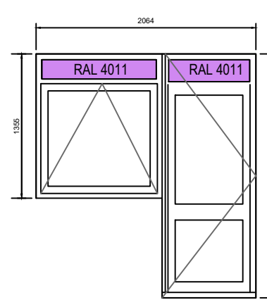
1 X Type J (L) Window
