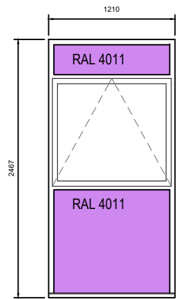
88 X Type A Window
