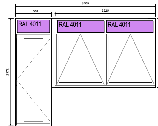
24 X Type G (R) Window
