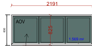
2 X Type D AOV Window
