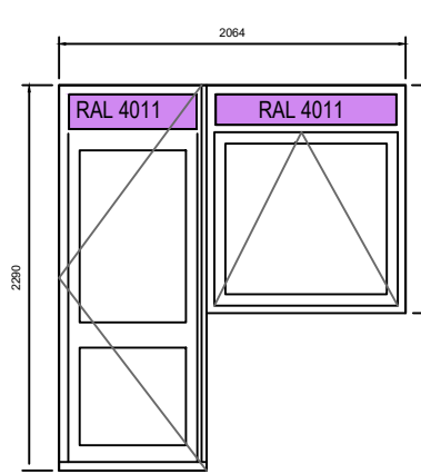
1 X Type J (R) Window
