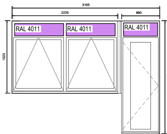
24 X Type G (L) Window
