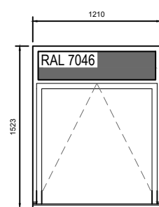
53 X Type H Window
