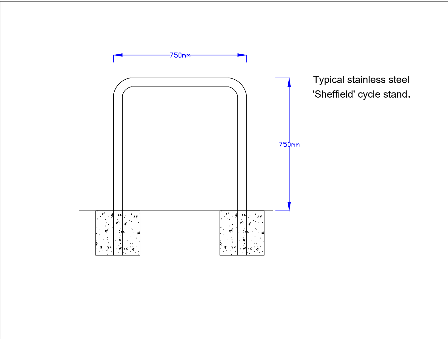
Typical Cycle Stand NTS
