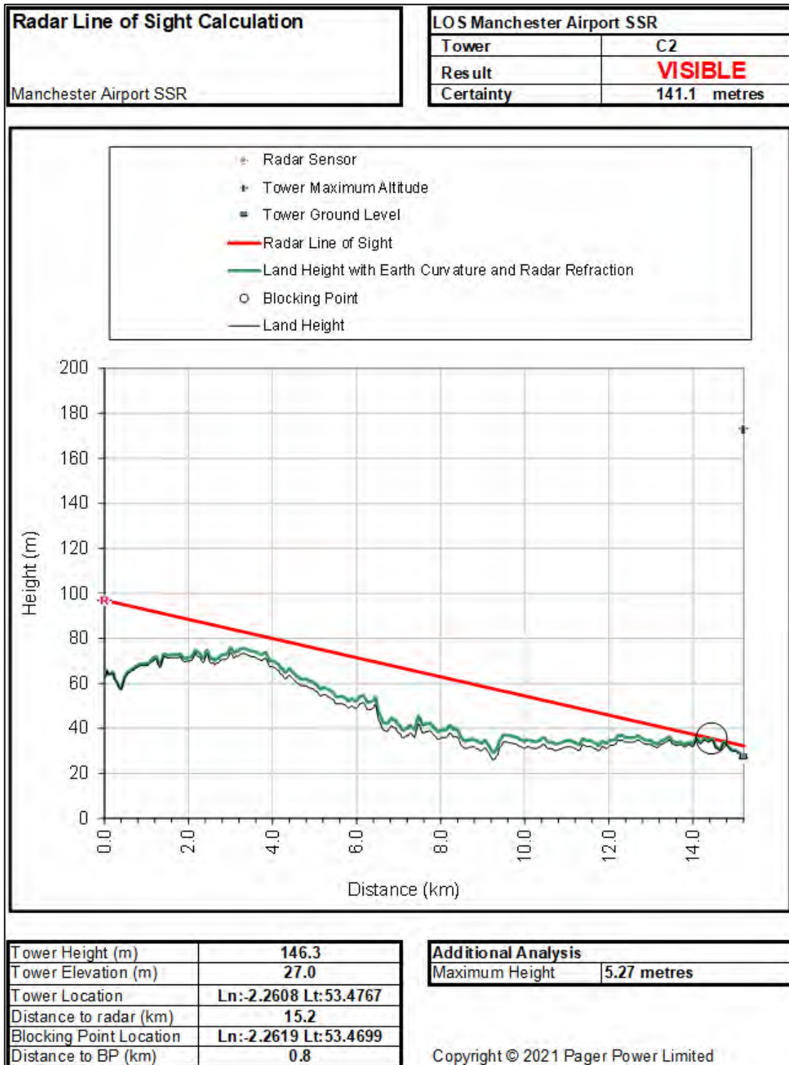
Figure 8 Manchester Airport SSR visibility for tower C2
