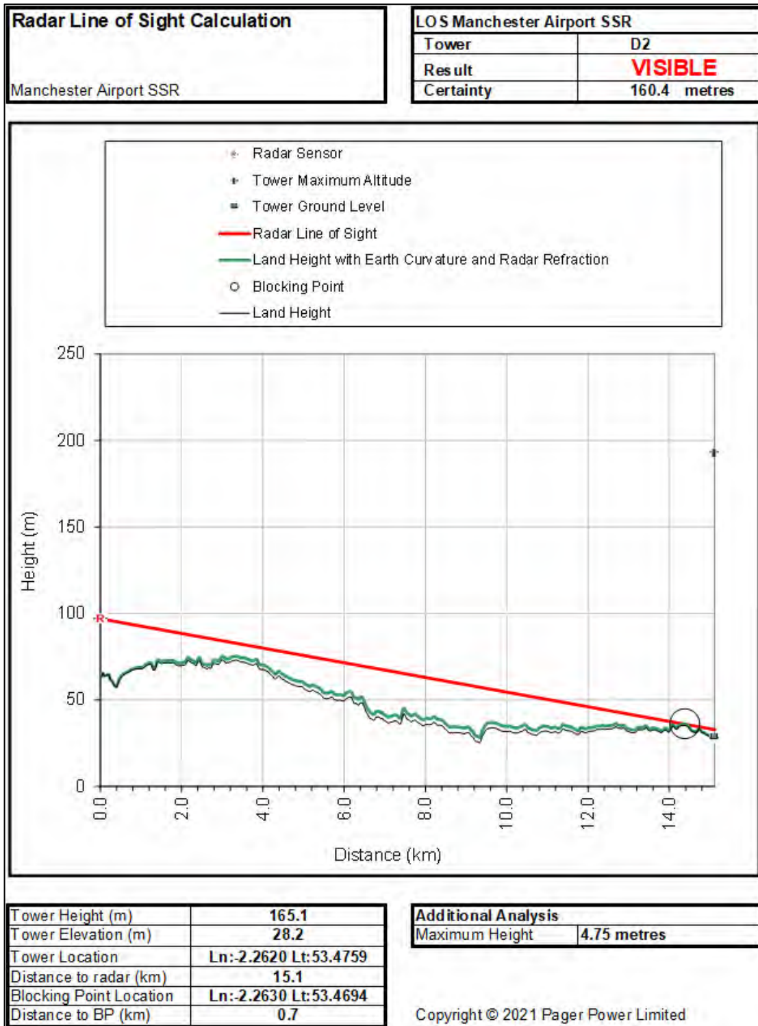
Figure 10 Manchester Airport SSR visibility for tower D2
