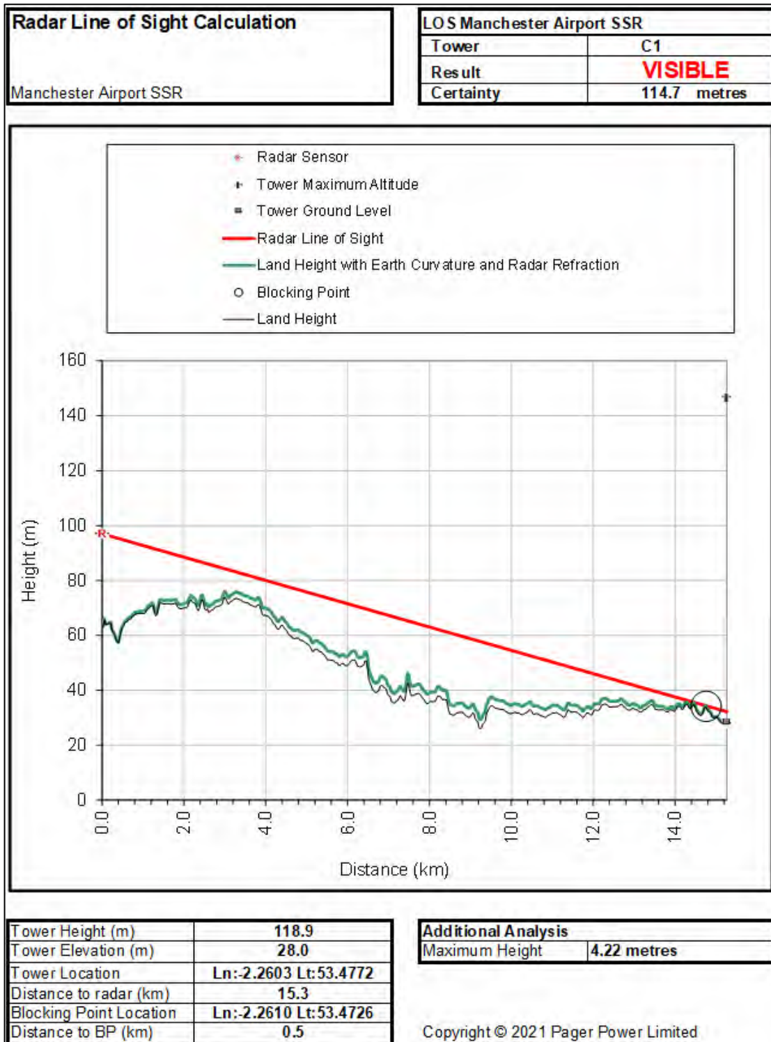
Figure 7 Manchester Airport SSR visibility for tower C1
