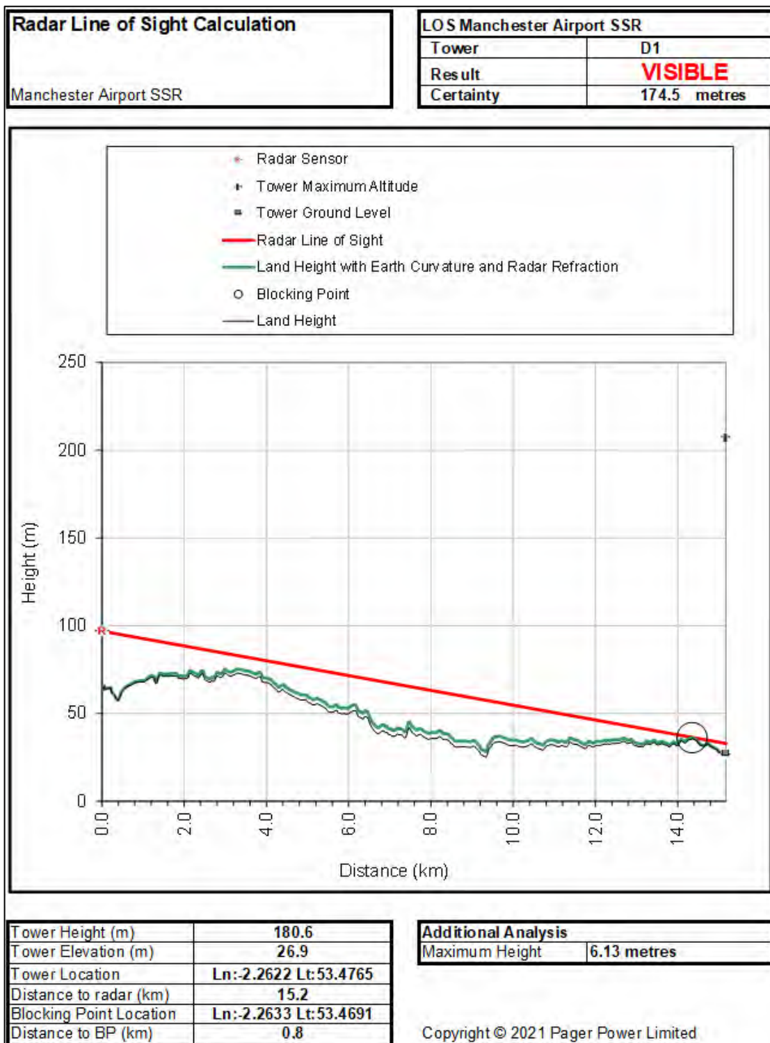
Figure 9 Manchester Airport SSR visibility for tower D1
