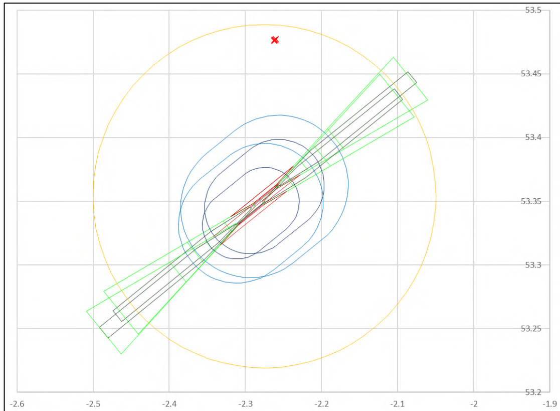
Figure 11 OLS chart
