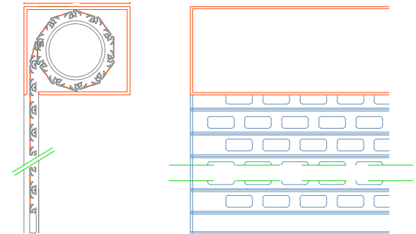
SHUTTER CURTAIN DETAIL
