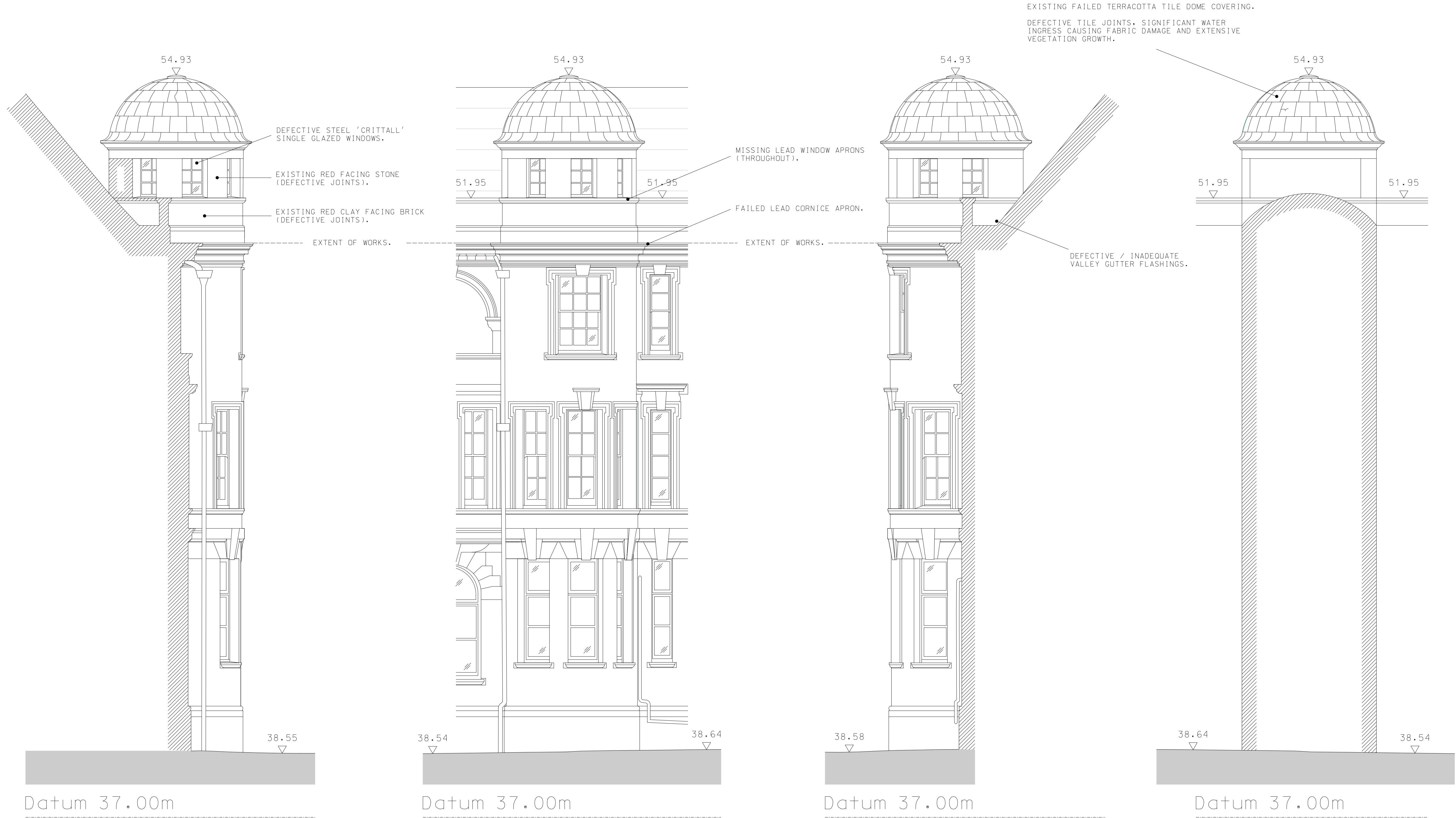
South Turret - Existing Elevations
