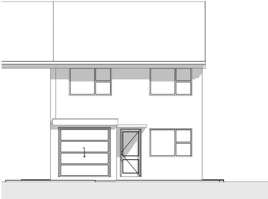
EXISTING NORTH WEST ELEVATION 1:100
