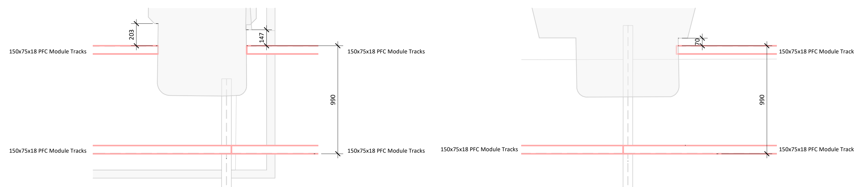
6 Lloyd St Secondary Steel Layout Detail A 1 : 20
