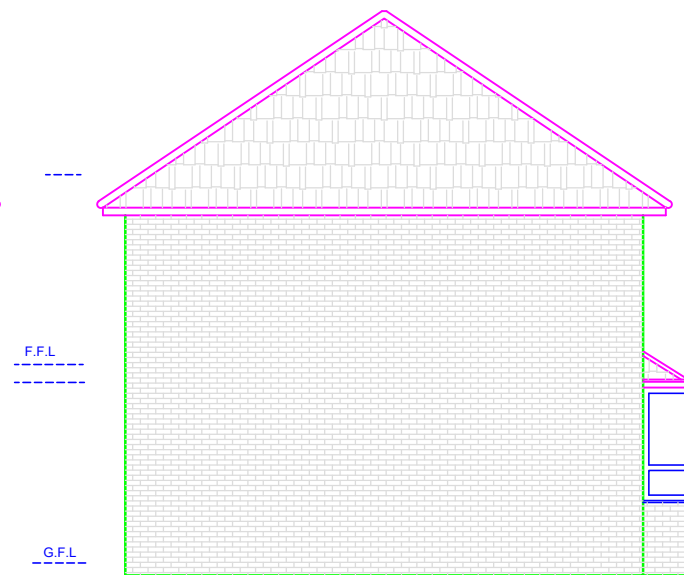
EXISTING SIDE ELEVATION(NORTH)
