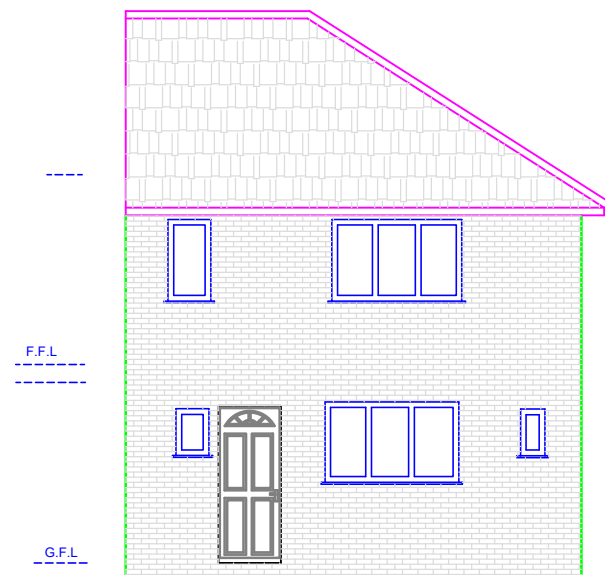
EXISTING REAR ELEVATION (EAST)
