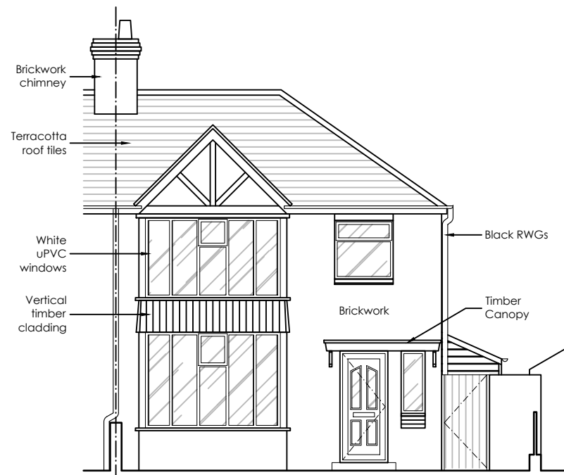
FRONT ELEVATION AS EXISTING
