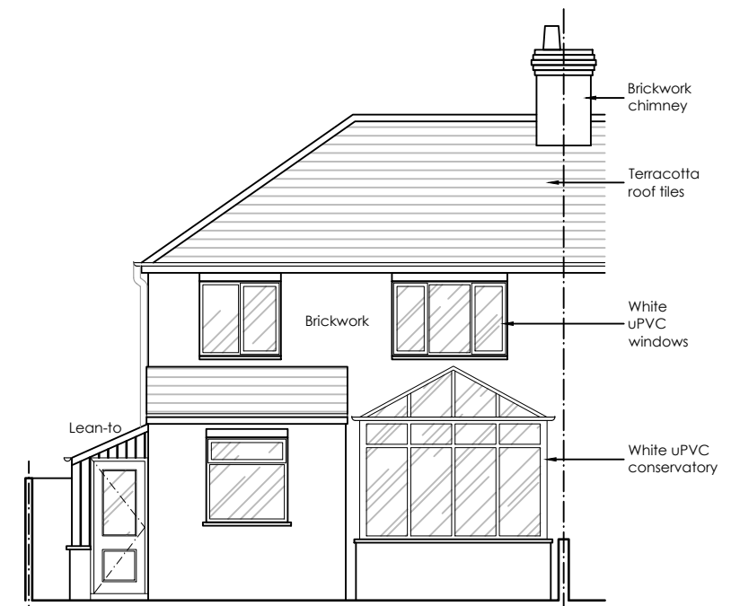
REAR ELEVATION AS EXISTING
