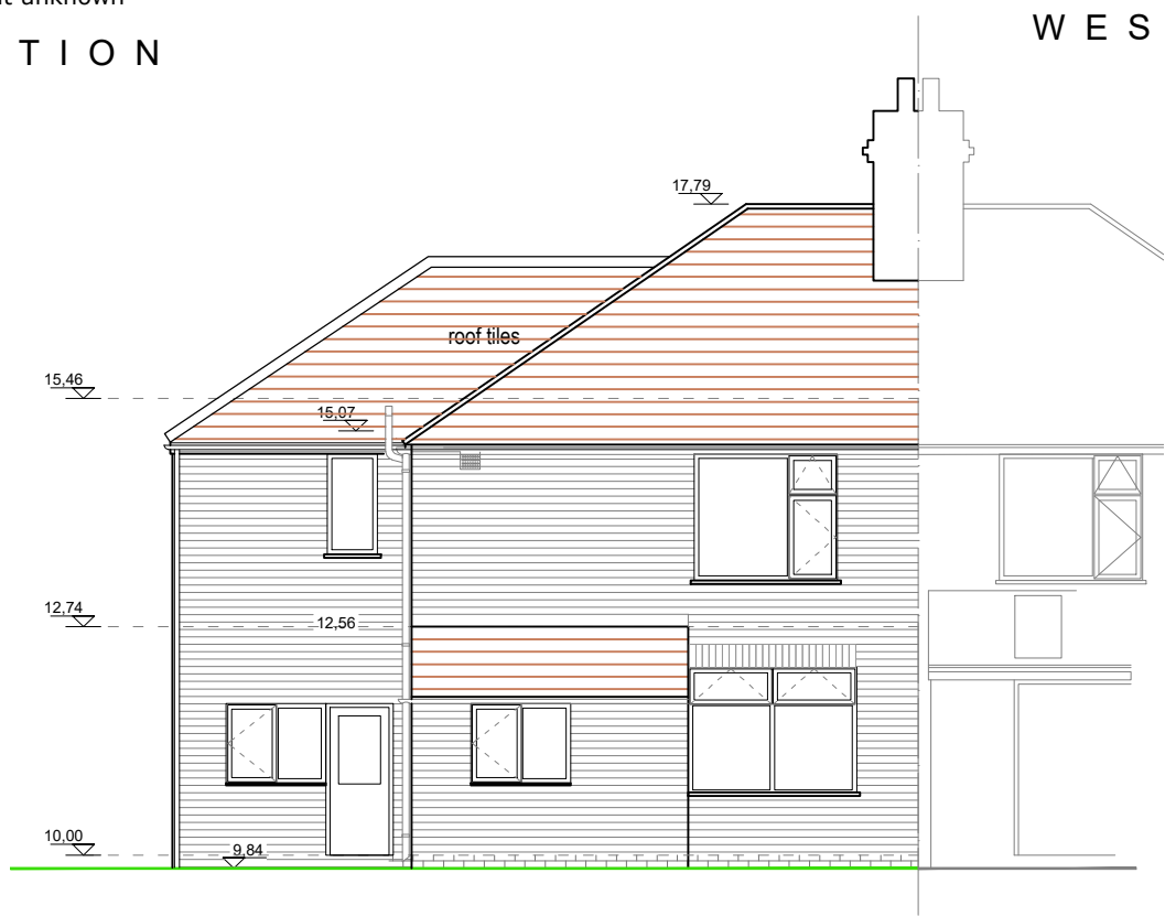
EAST ELEVATION
