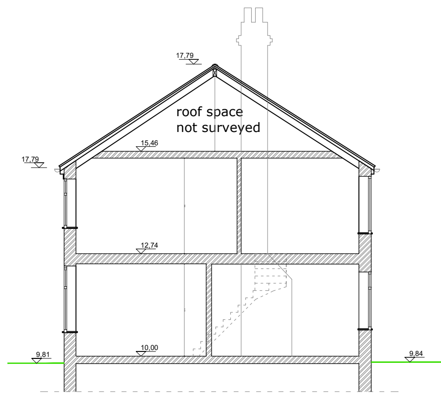
CROSS SECTION
