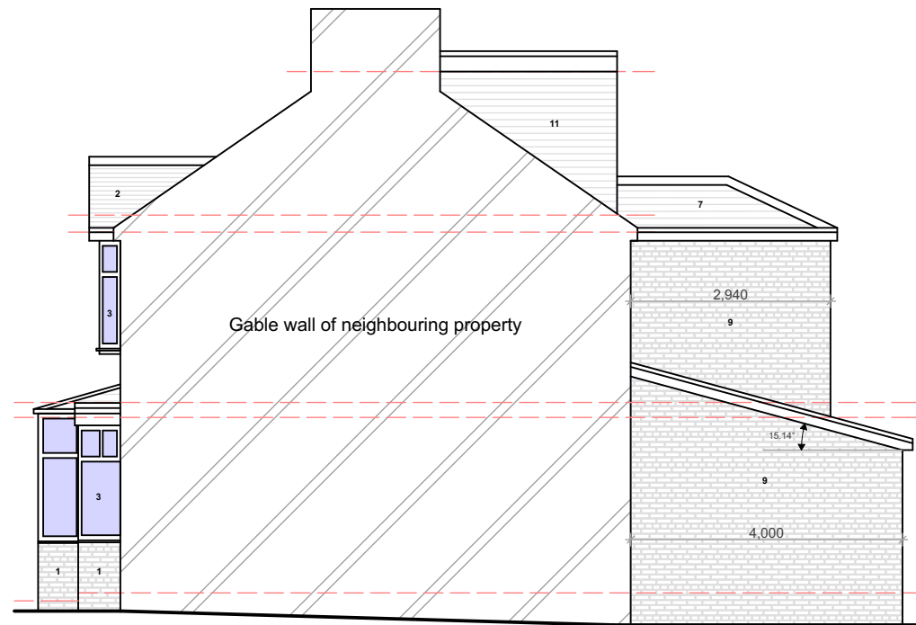
PROPOSED GA SIDE ELEVATION 2 @1:100
