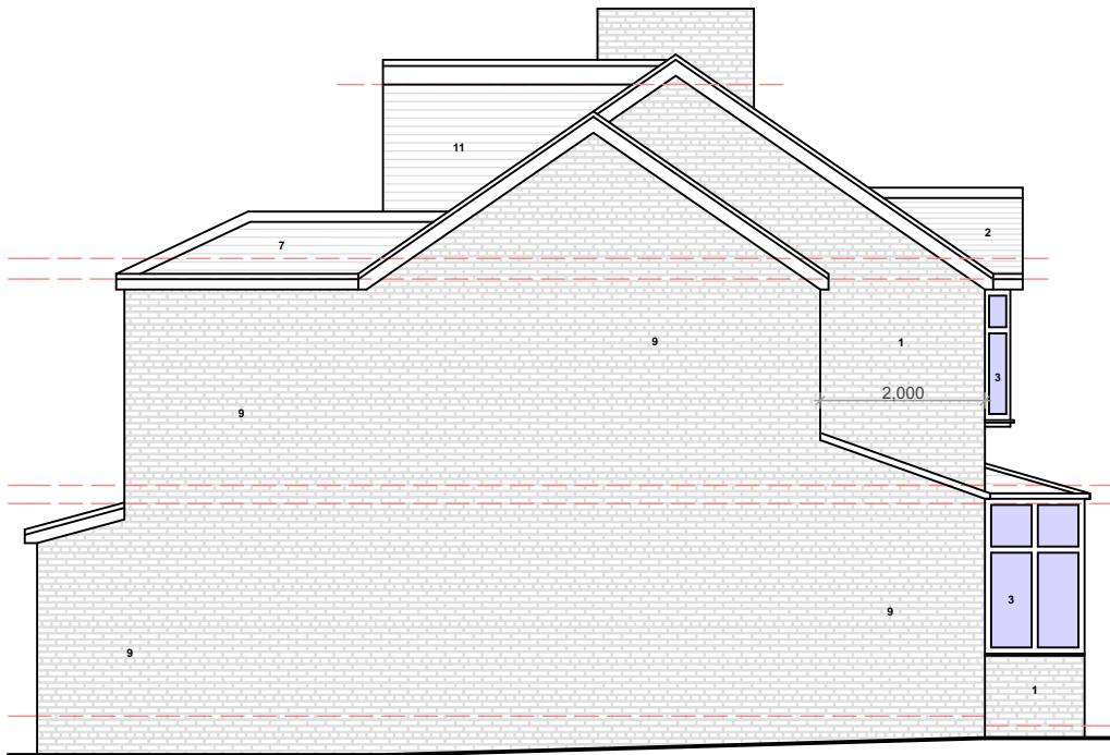
PROPOSED GA SIDE ELEVATION 1 @1:100
