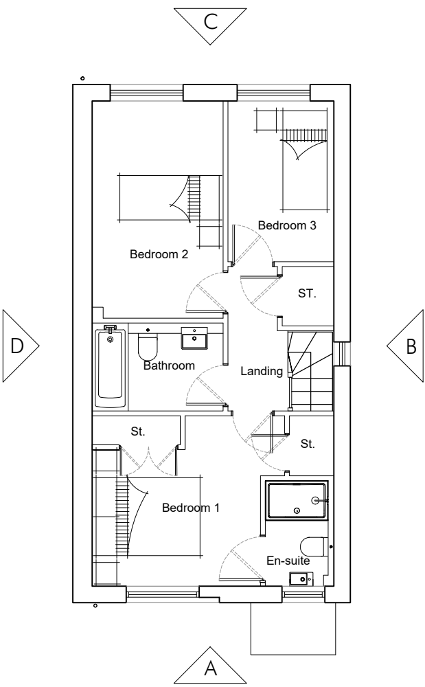
First Floor 43 Sq.m/468 Sq.ft
